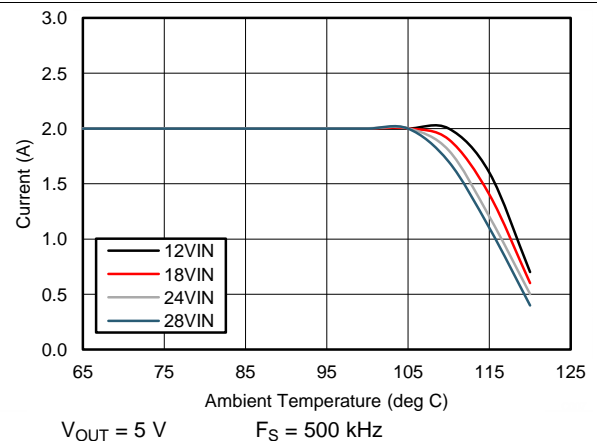
Figure 62. Derating Curve
