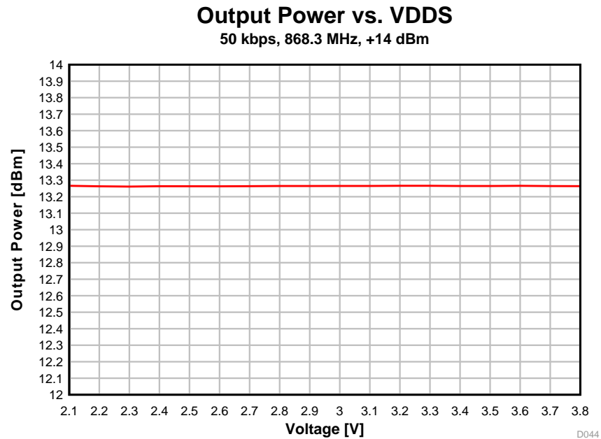
图 5-17. Output Power vs. Supply Voltage (VDD5) (50 kbps, 868.3 MHz)
