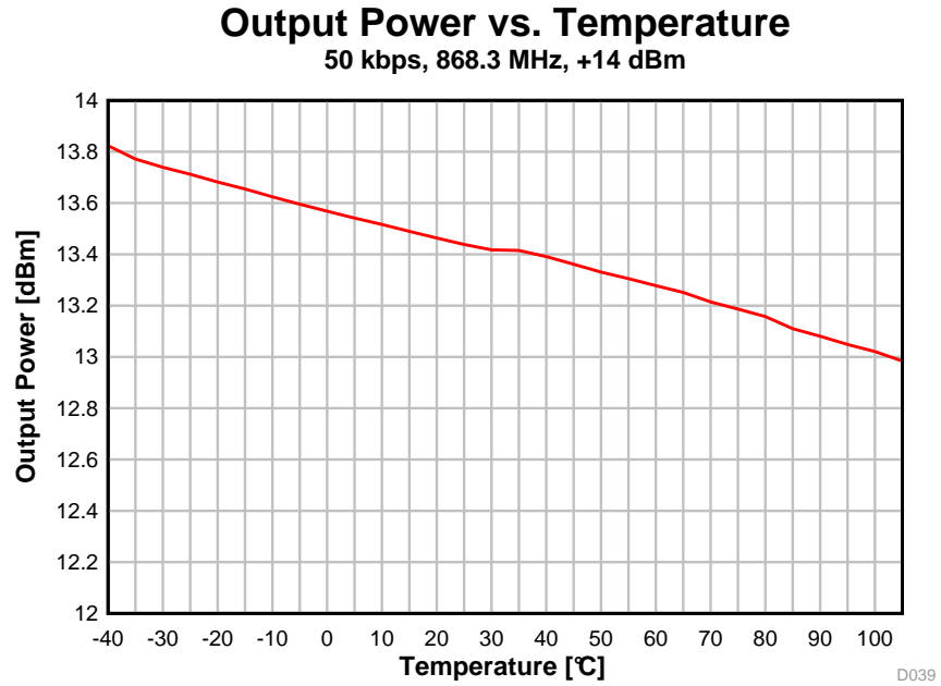
图 5-16. Output Power vs. Temperature (50 kbps, 868.3 MHz)
