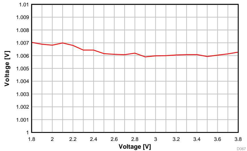
图 5-25. ADC Accuracy vs. Supply Voltage (VDD5)
