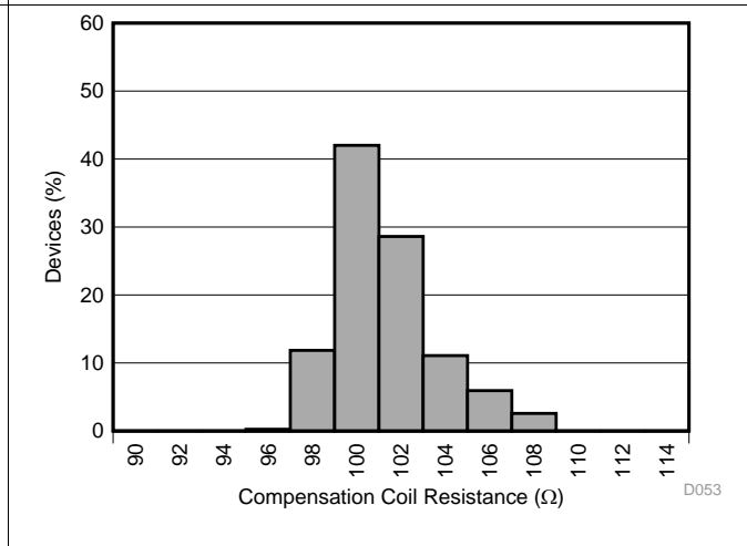
图 16. Compensation Coil Resistance Histogram
