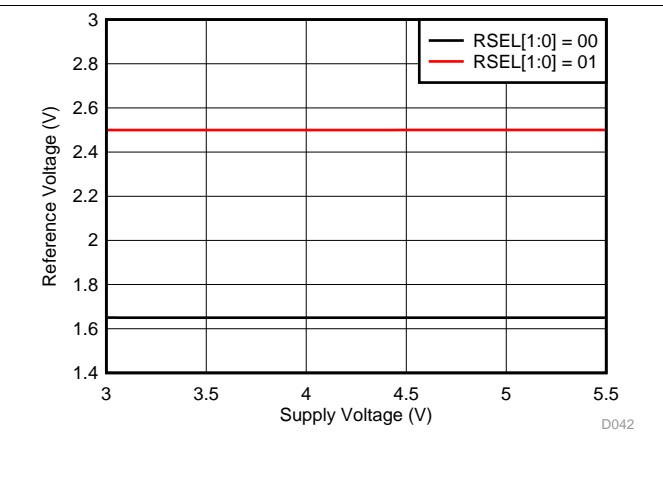
图 50. Reference Voltage vs Supply Voltage
