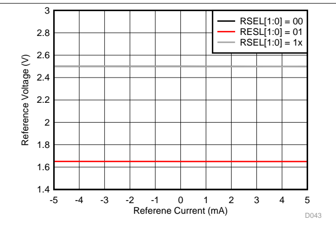
图 52. Reference Voltage vs Reference Output Current
