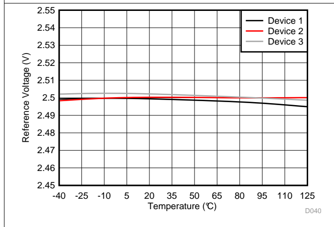
图 51. Reference Voltage vs Temperature
