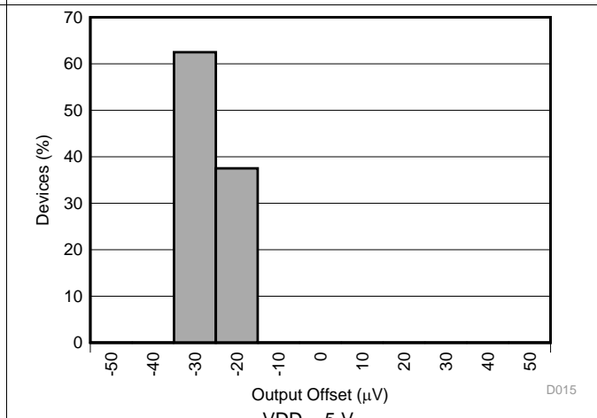
图 18. Shunt-Sense Amplifier Output Offset Histogram
