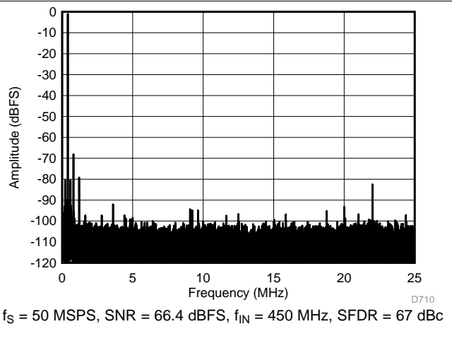
Figure 109. FFT for 450-MHz Input Signal (Dither Off)
