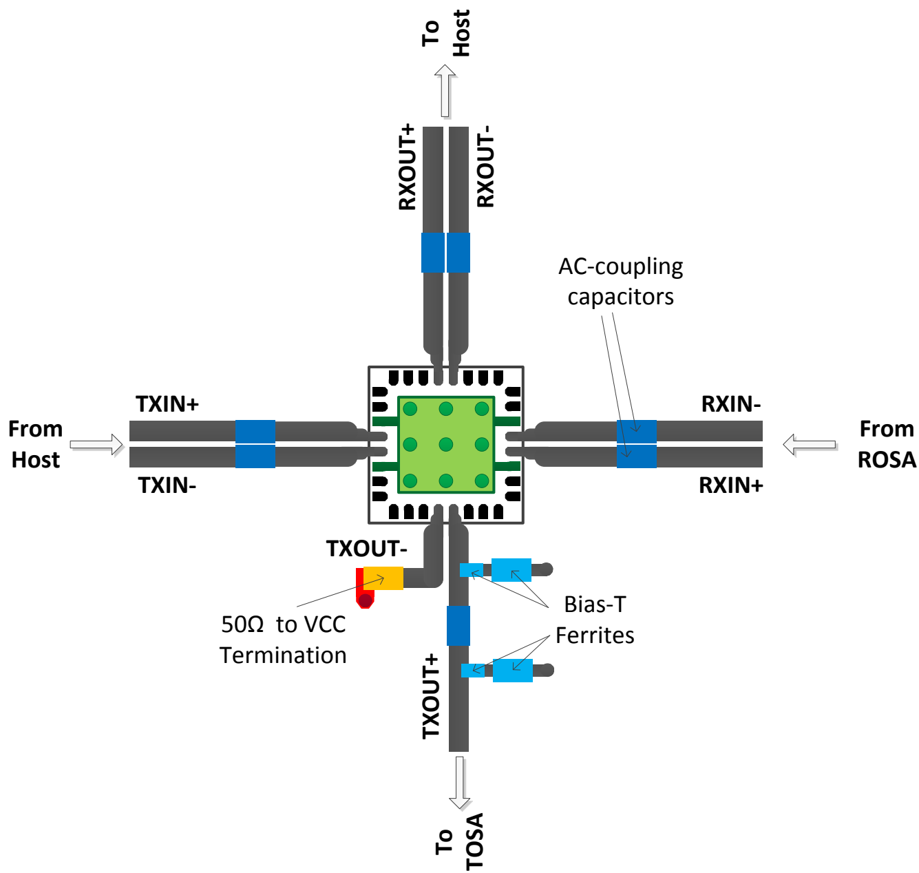
图 69. Board Layout
