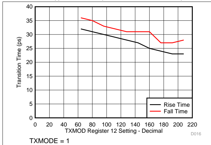
Figure 8. TX Rise-Time and Fall-Time vs Modulation Current
