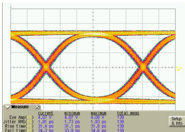
图 65. Differential Mode Transmitter Output Eye Diagram
