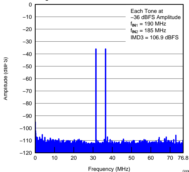
Figure 13. AMPLITUDE vs FREQUENCY (Two-Tone Input Signal)
