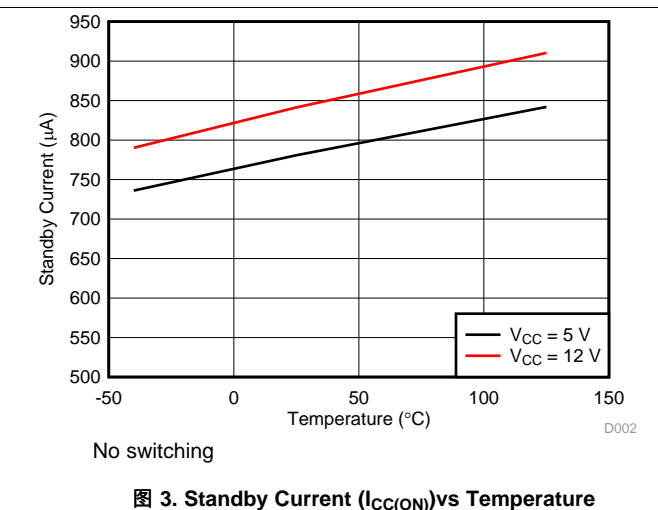
图 3. Standby Current ( I_{\text{CC(ON)}} ) vs Temperature
