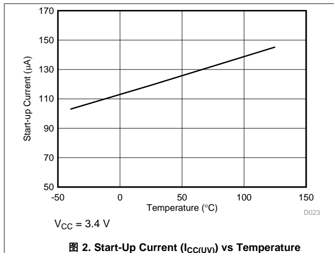
图 2. Start-Up Current ( I_{\text{CC(UV)}} ) vs Temperature
