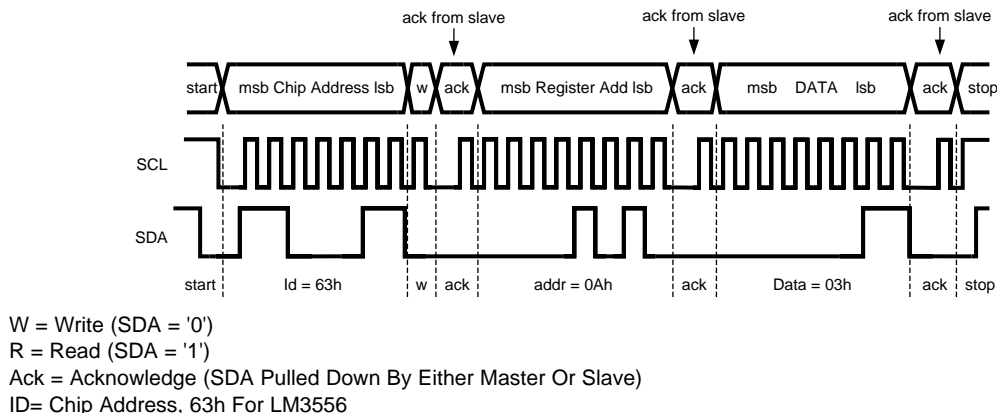
Figure 31. Write Cycle
