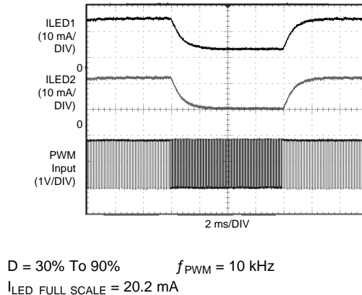
Figure 20. Response To Step Change in PWM Input Duty Cycle
