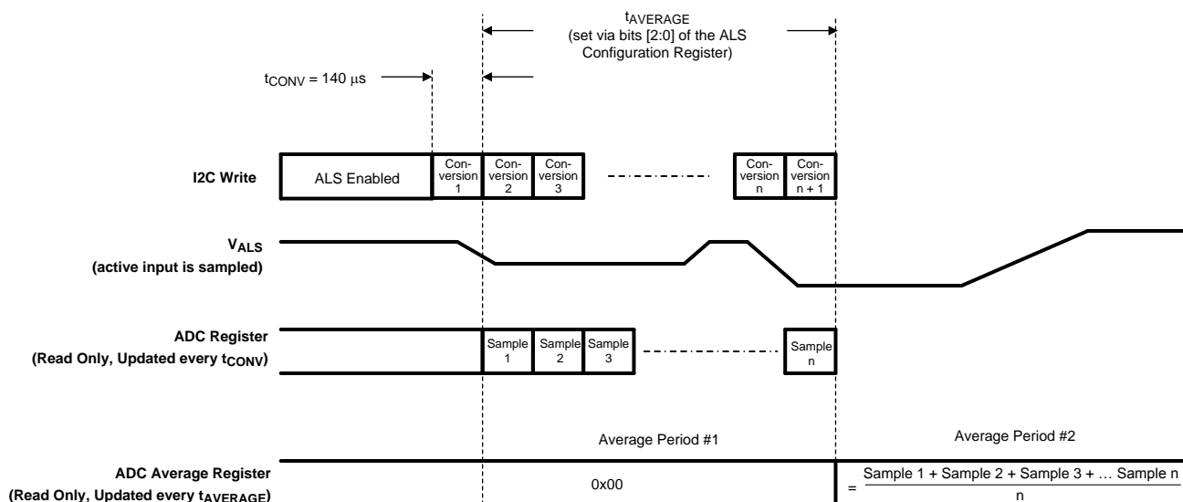
Figure 28. ADC Timing
