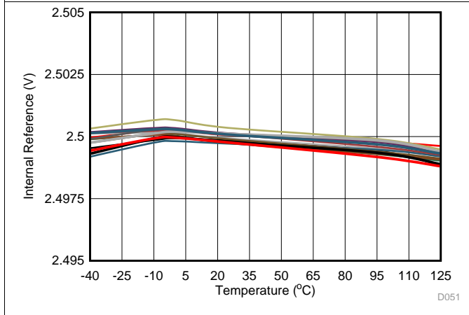
Figure 53. Internal Reference Voltage vs Temperature
