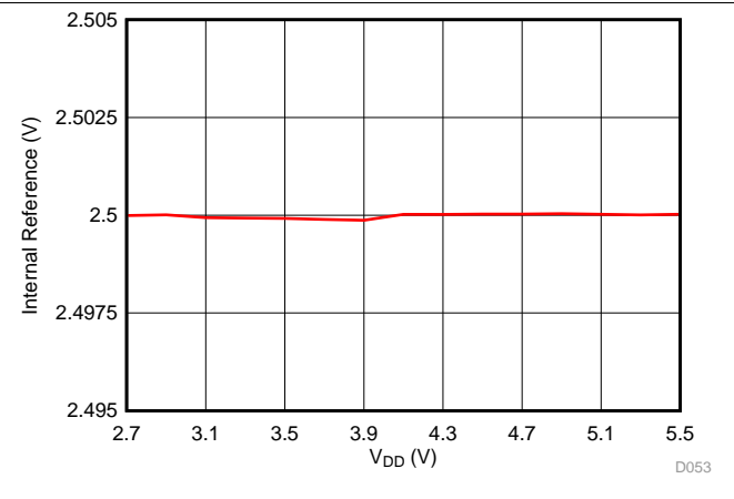
Figure 54. Internal Reference Voltage vs Supply Voltage
