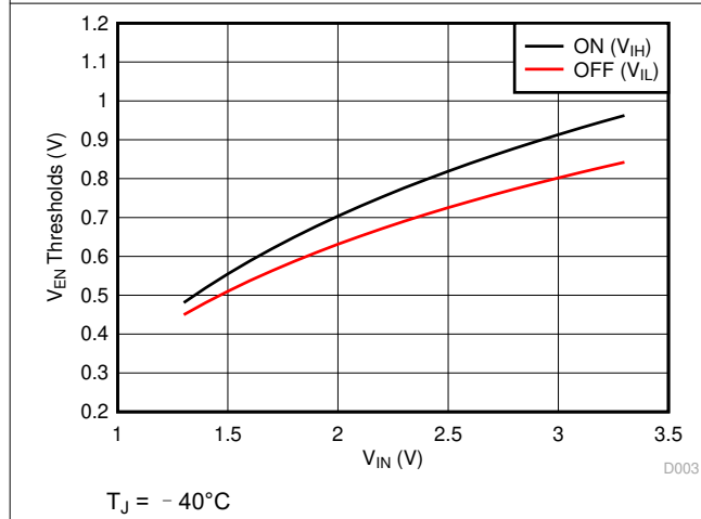
图 6-3. V_{EN} Thresholds vs V_{IN}
