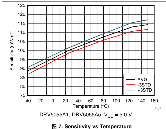
图 7. Sensitivity vs Temperature
