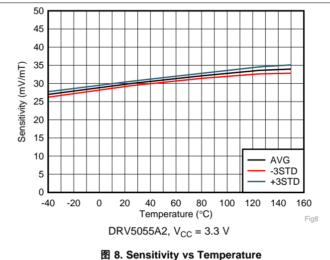
图 8. Sensitivity vs Temperature
