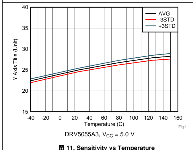
图 11. Sensitivity vs Temperature
