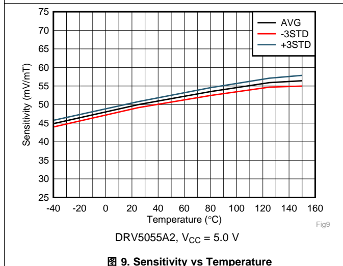
图 9. Sensitivity vs Temperature
