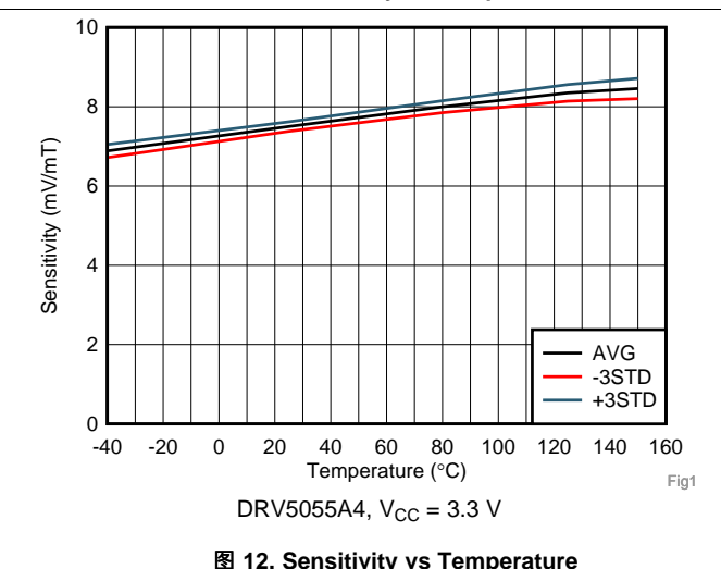
图 12. Sensitivity vs Temperature
