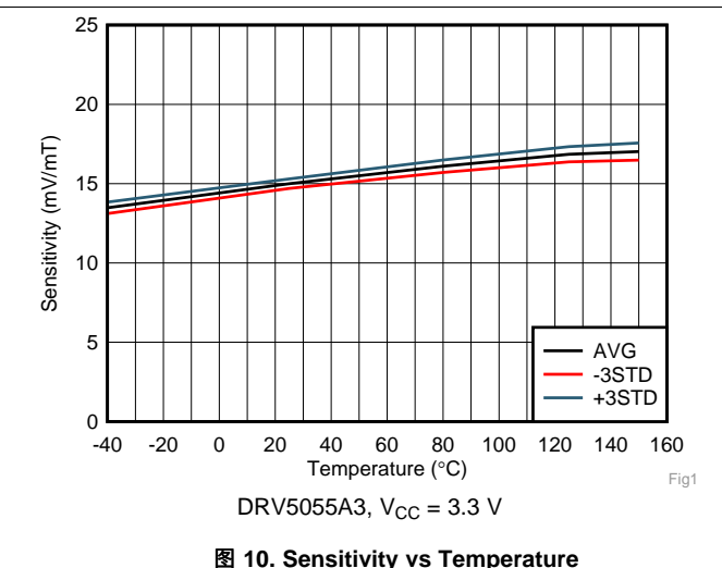
图 10. Sensitivity vs Temperature
