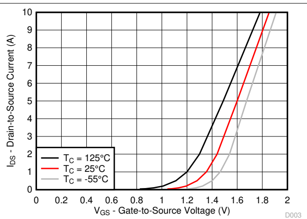
图 5-3. Transfer Characteristics
