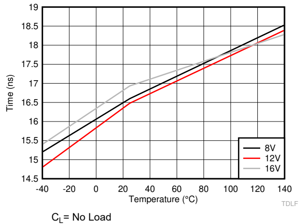
图 6-25. LO Falling Propagation Delay (TDLFF)
