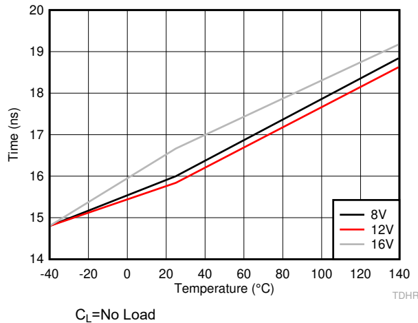
图 6-22. HO Rising Propagation Delay (TDHRR)
