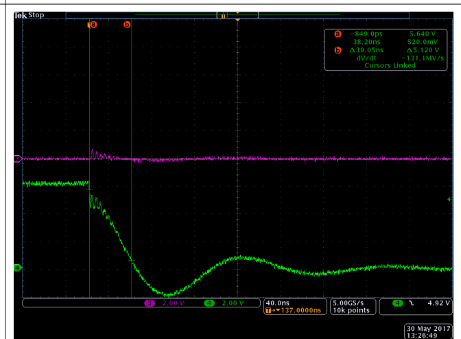
V_{DD}=V_{HB}=6\text{ V} , HS=V_{SS} C_{LOAD}=10\text{ nF} Ch4=LO
