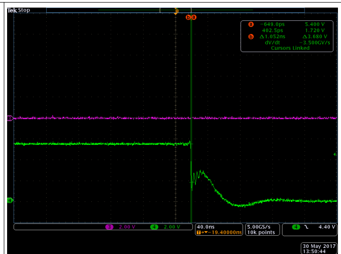
V_{DD}=V_{HB}=6\text{ V} , HS=V_{SS} C_{LOAD}=10\text{ nF} Ch4=HO
