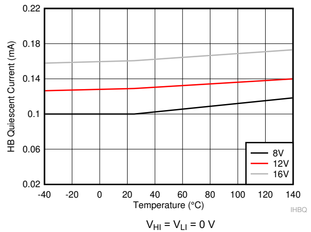
图 6-3. HB Quiescent Current
