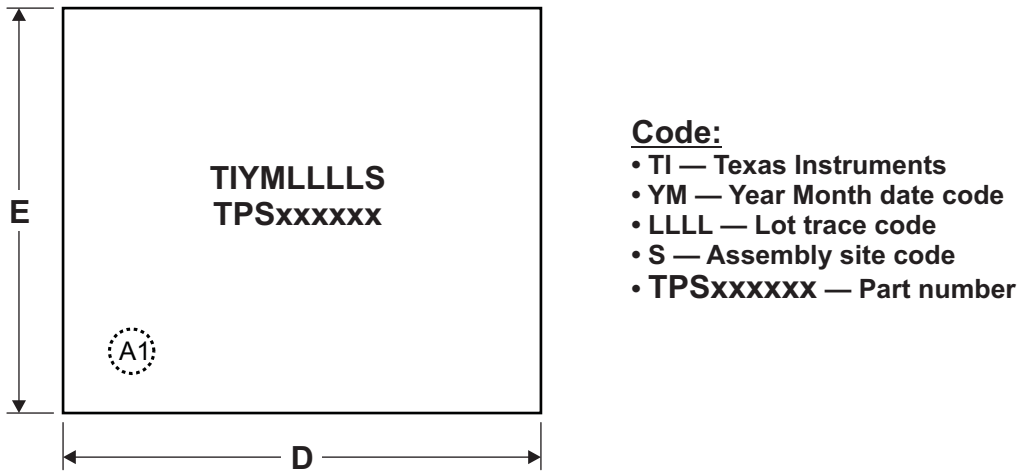
Figure 54. Package Marking and Dimensions
