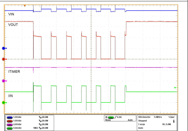
图 9-18. Overload Response and Recovery
