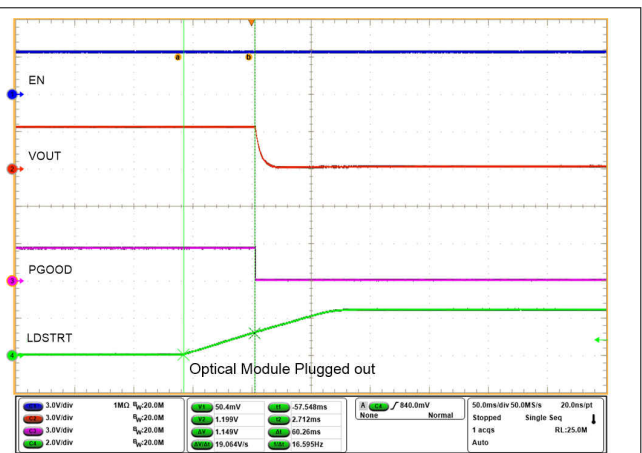
图 9-16. Output Voltage Profile When Optical Module is Plugged Out
