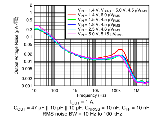
图 11. Output Noise vs Frequency and Input Voltage
