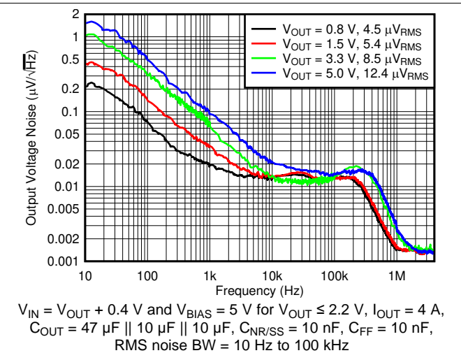
图 10. Output Noise vs Frequency and V_{OUT}
