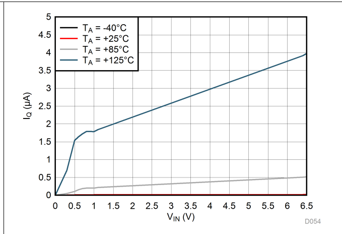
Figure 14. LP5912-0.9 I_{Q(SD)} vs V_{IN}
