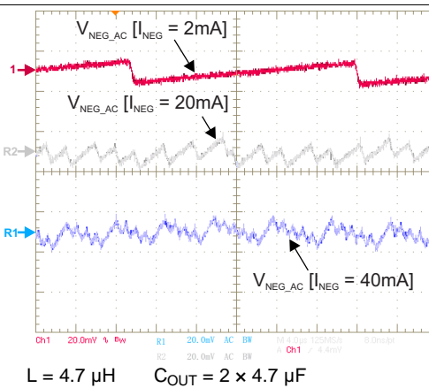
Figure 25. V_{\text{NEG}} Output Voltage Ripple — 40mA Mode
