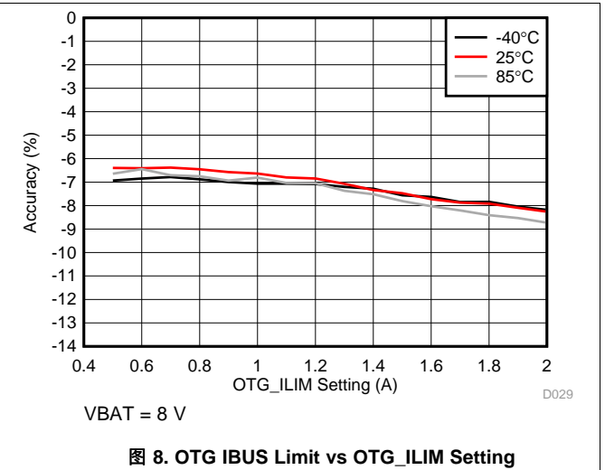
图 8. OTG IBUS Limit vs OTG_ILIM Setting
