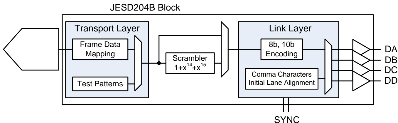
Figure 157. JESD204B Block
