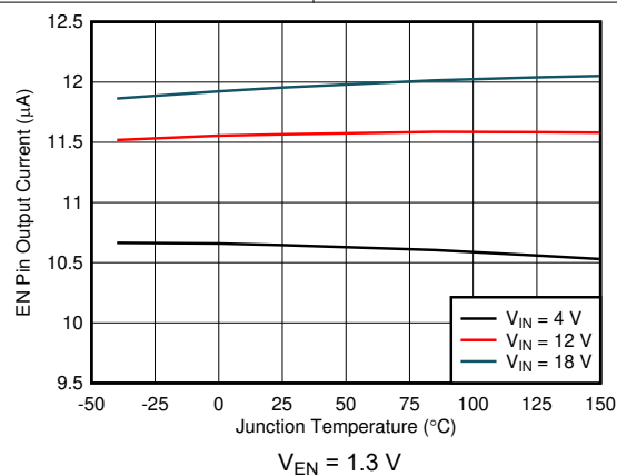
图 6-11. EN Pin Current vs Junction Temperature
