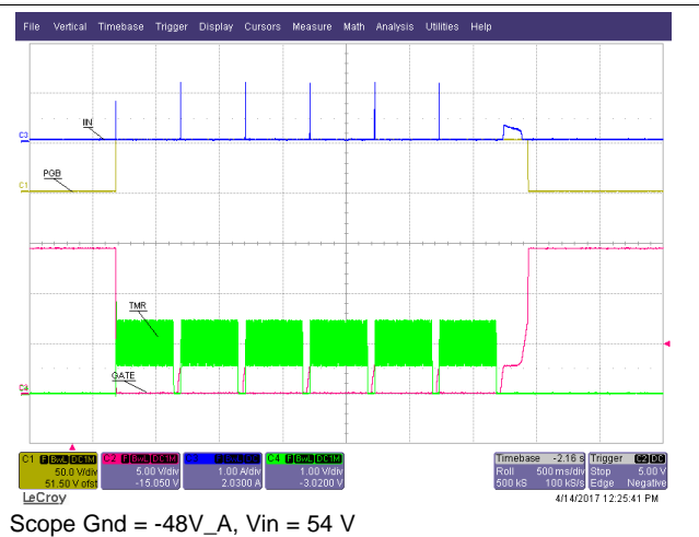
Figure 34. Apply Short and Remove Short
