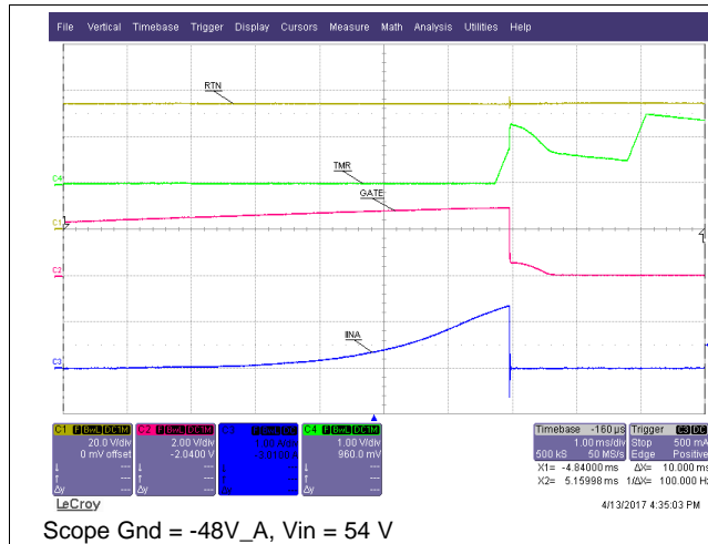
Figure 33. Start Into Short
