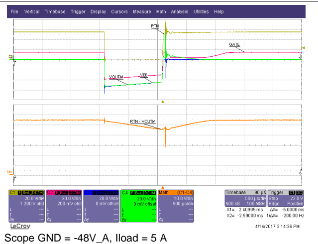
Figure 36. 1-ms Brown Out
