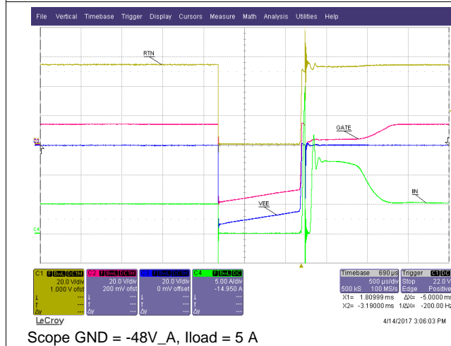
Figure 35. 1-ms Brown Out
