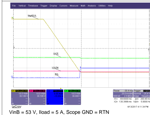
Figure 37. Supply Switch Over (Raise VinA)
