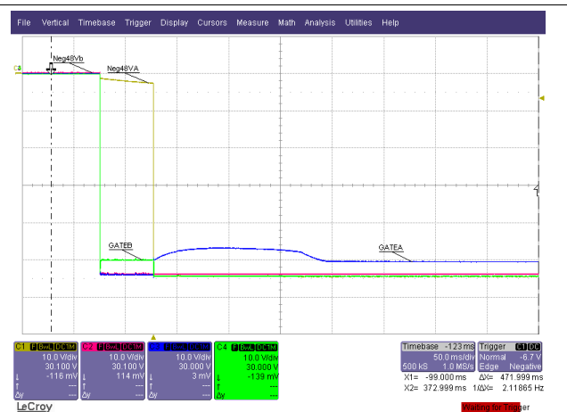
VinA = 54.5 V, VinB = 54 V, No Load, Scope GND = RTN
