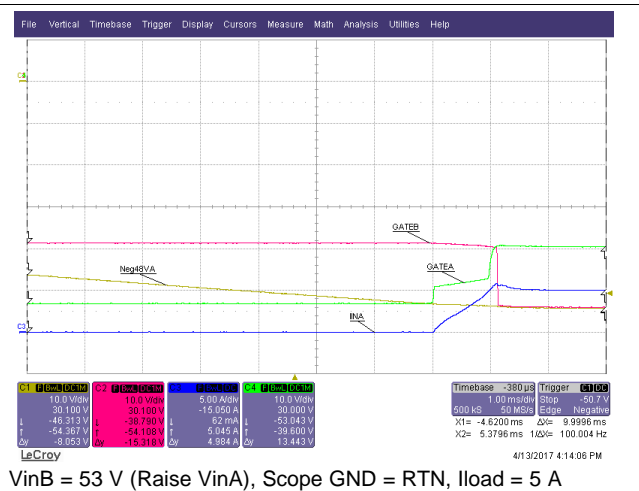
Figure 38. Supply Switch Over (zoomed in)
