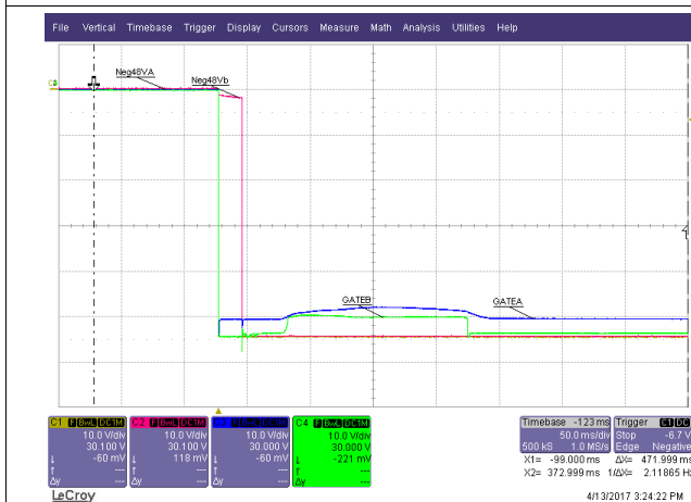
VinA = 54 V, VinB = 54 V, No Load, Scope GND = RTN
