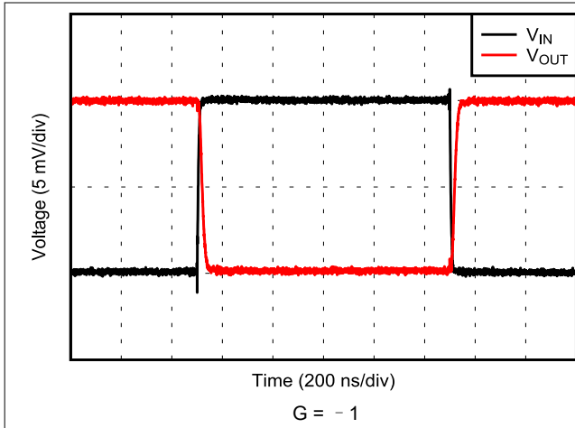
图 6-32. Small-Signal Step Response
