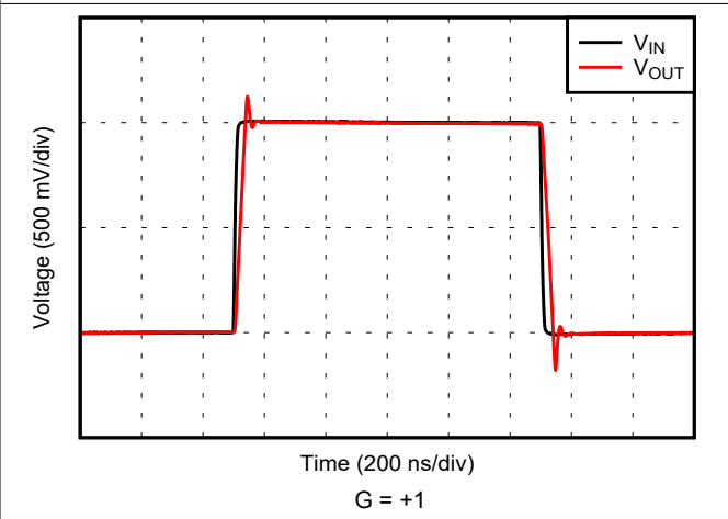
图 6-35. Large-Signal Step Response
