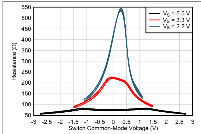
图 6-44. Switch On-Resistance vs Common-Mode Voltage
