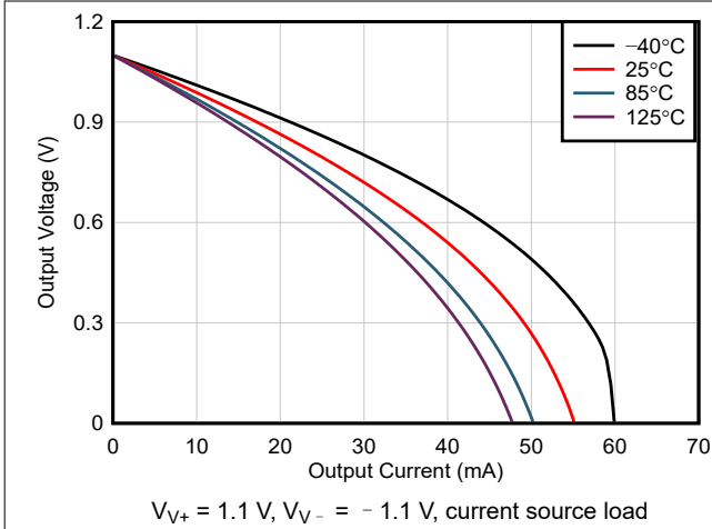
图 6-20. Output Voltage Swing vs Output Current
