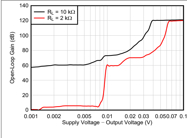
图 6-26. Open-Loop Gain vs Output to Supply Voltage Delta
