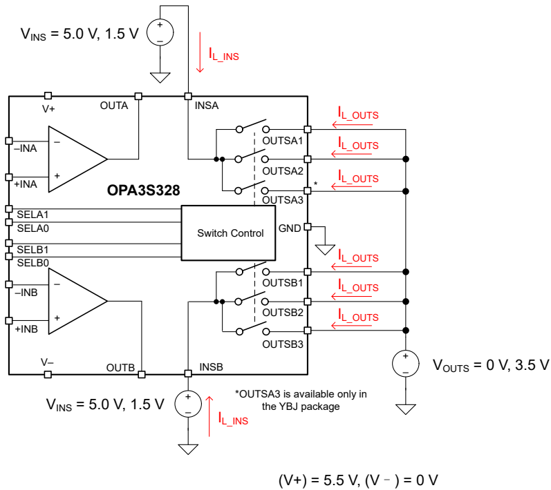
图 7-1. Switch Leakage Current, Open
