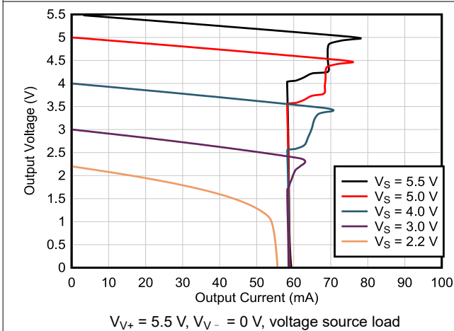
图 6-24. Output Voltage Swing vs Output Current
