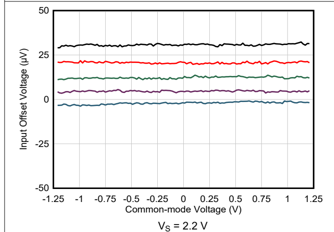
图 6-6. Offset Voltage vs Common-Mode Voltage
