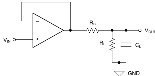
图 9-1. Improving Capacitive Load Drive
