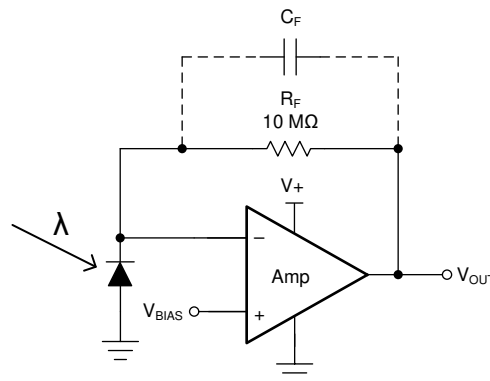
图 9-4. Single-Supply Transimpedance Amplifier
