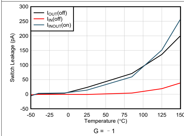
图 6-36. Switch Leakage Current vs Temperature
