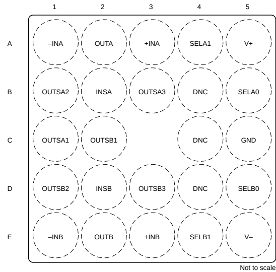
图 5-2. OPA3S328 YBJ (24-Pin DSBGA Preview) Package, Top View
