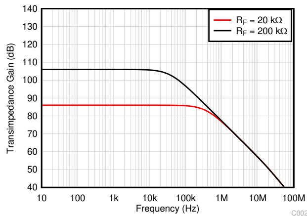
图 9-6. OPA3S328 Transimpedance Gain
