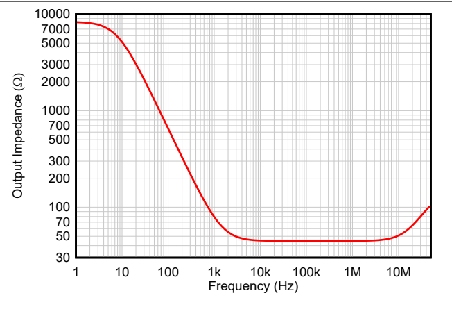
图 6-25. Open-Loop Output Impedance vs Frequency
