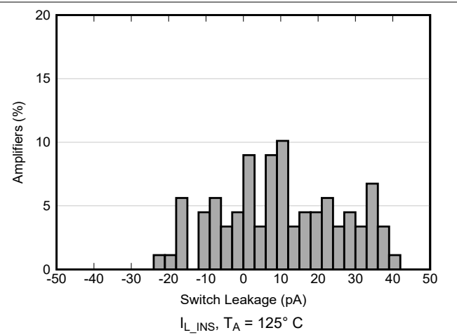
图 6-39. Switch Input Leakage Current Histogram
