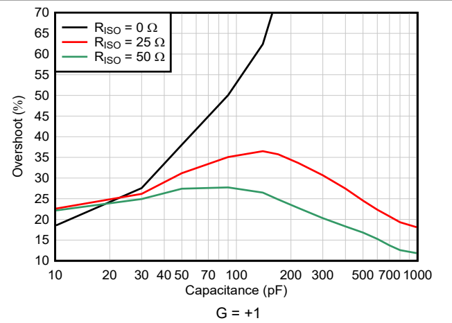
图 6-29. Small-Signal Overshoot vs Load Capacitance
