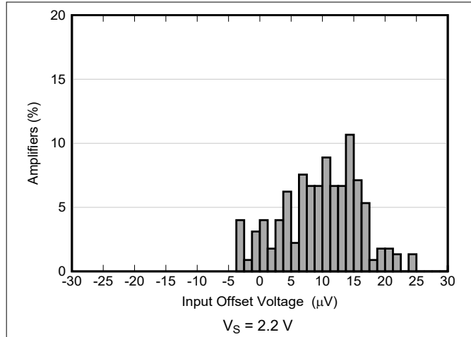
图 6-2. Offset Voltage Production Distribution
