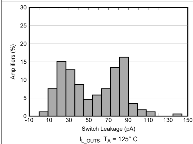
图 6-42. Switch Output Leakage Current Histogram
