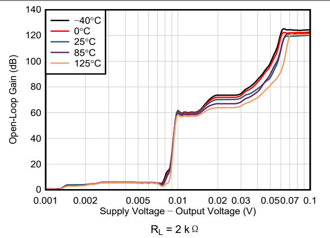
图 6-27. Open-Loop Gain vs Output to Supply Voltage Delta
