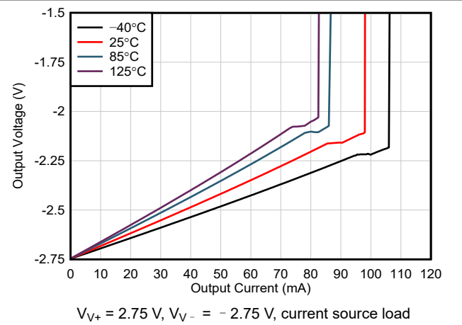
图 6-23. Output Voltage Swing vs Output Current
