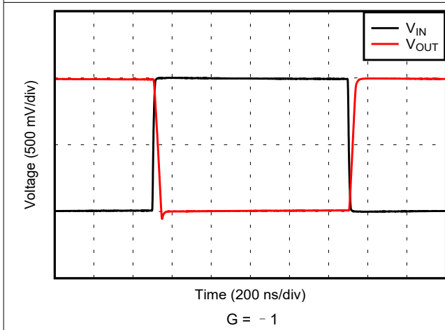
图 6-34. Large-Signal Step Response
