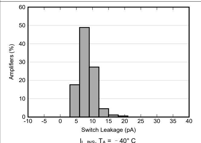
图 6-37. Switch Input Leakage Current Histogram
