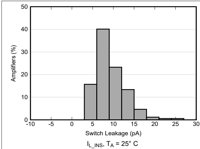
图 6-38. Switch Input Leakage Current Histogram
