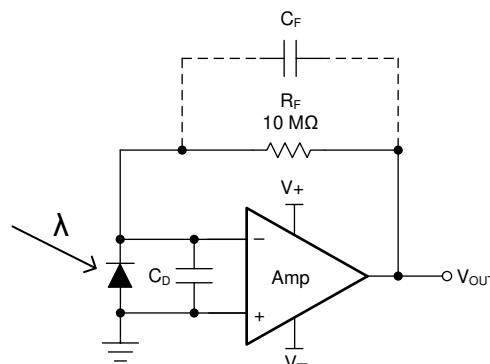
图 9-3. Dual-Supply Transimpedance Amplifier
