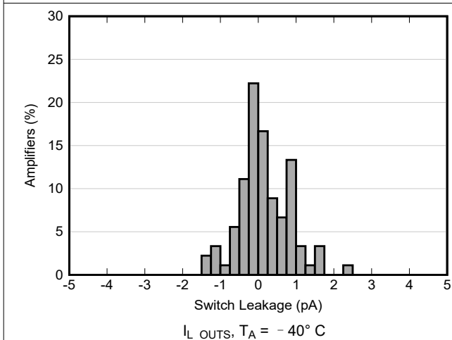
图 6-40. Switch Output Leakage Current Histogram
