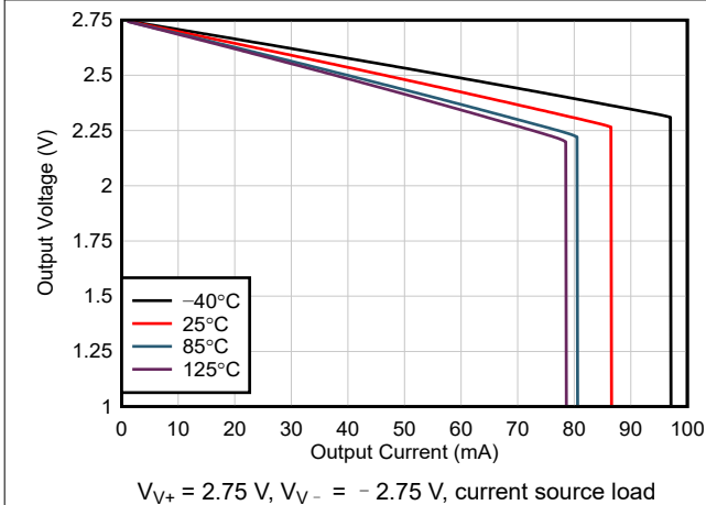
图 6-22. Output Voltage Swing vs Output Current
