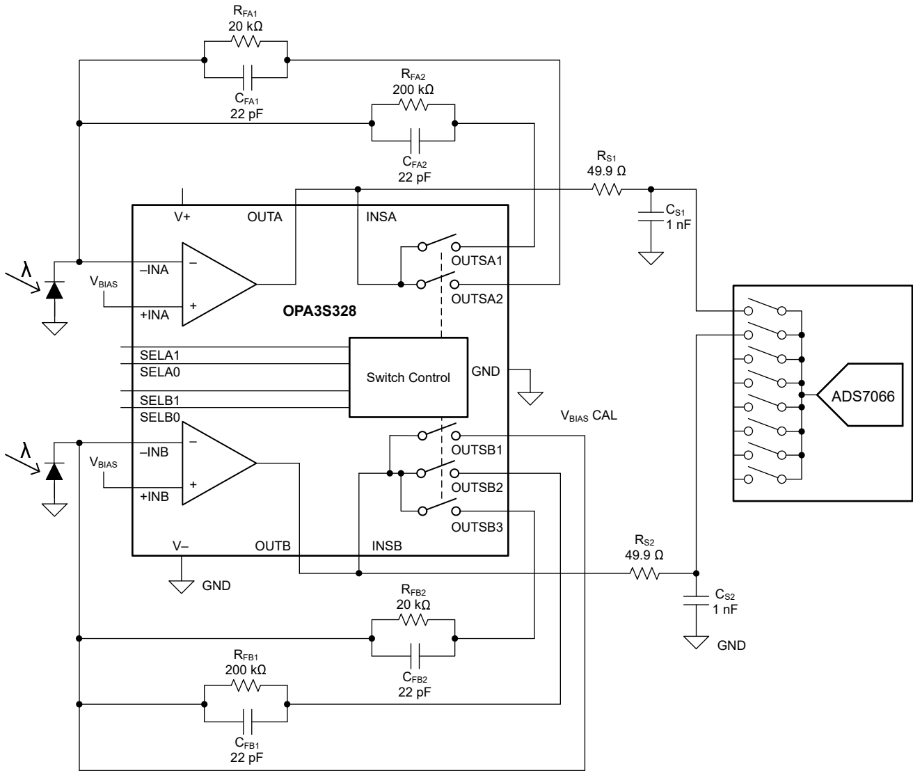
图 9-5. Dual Transimpedance Front End With Gain Switching
