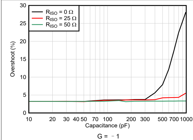
图 6-28. Small-Signal Overshoot vs Load Capacitance
