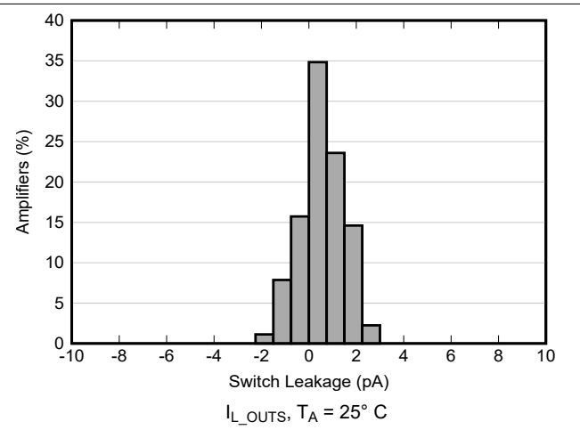
图 6-41. Switch Output Leakage Current Histogram
