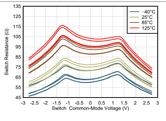
图 6-43. Switch On-Resistance vs Common-Mode Voltage
