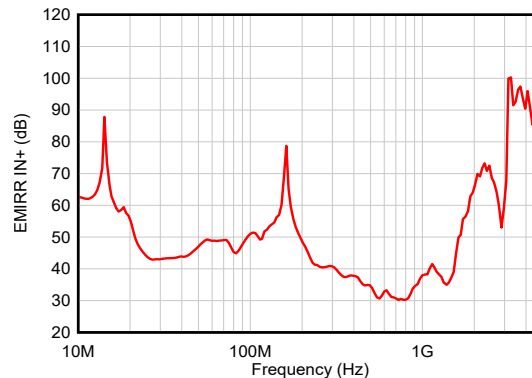
图 9-2. OPA3S328 EMIRR Response
