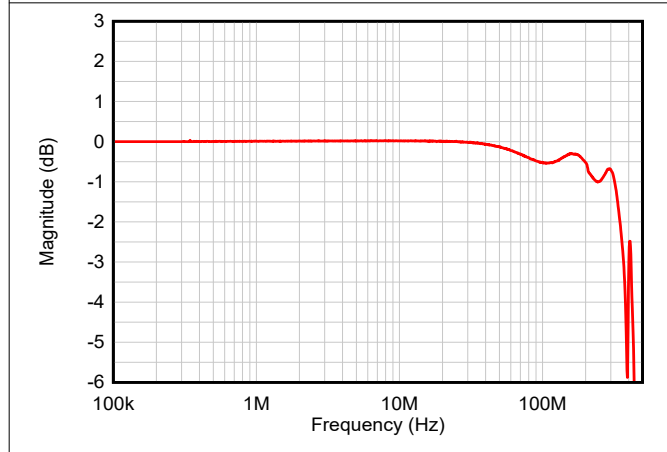
图 6-46. Switch Attenuation vs Frequency
