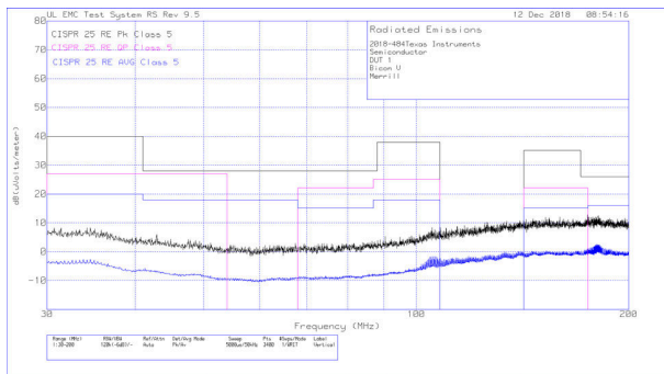
图 9-23. Radiated EMI Biconical Antenna (Vertical)
