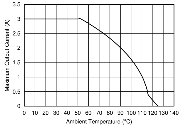
Figure 9-4. Maximum Output Current vs Ambient Temperature
