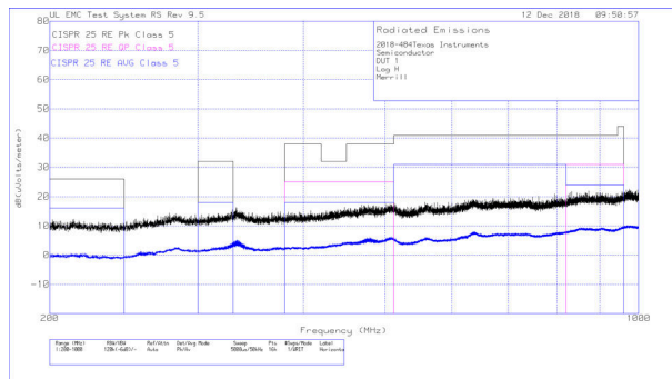
图 9-24. Radiated EMI Log-Periodic Antenna (Horizontal)
