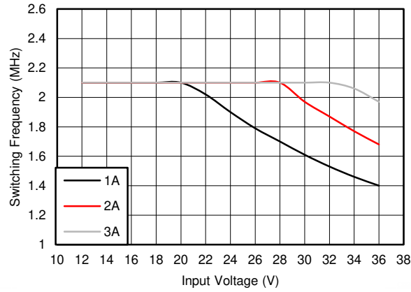
图 8-13. Switching Frequency vs Input Voltage V_{OUT} = 3.3 V
