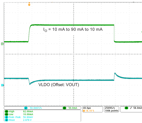
图 9-18. LDO6, LDO8 Load Transient Response
