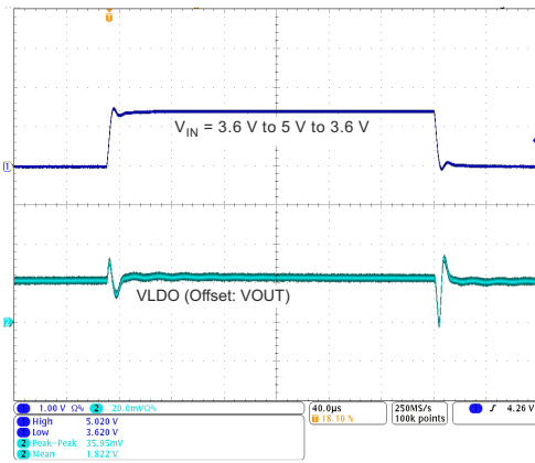
图 9-19. LDO6, LDO8 Line Transient Response
