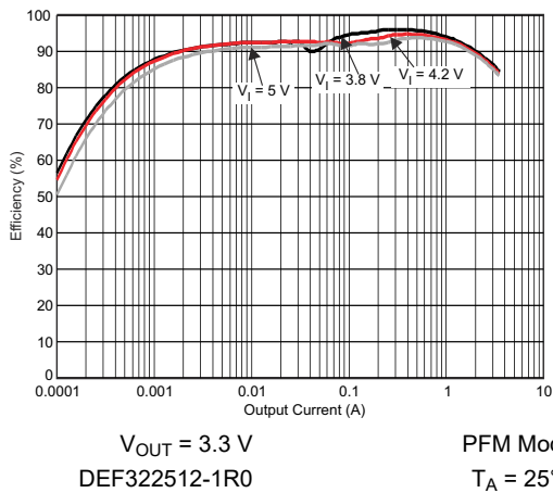
图 6-21. DCDC4 Efficiency vs Output Current
