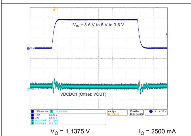
图 9-6. DCDC1 Line Transient Response
