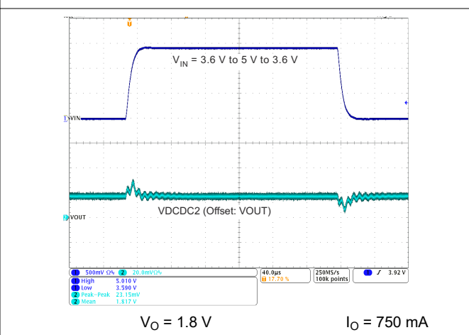
图 9-7. DCDC2 Line Transient Response
