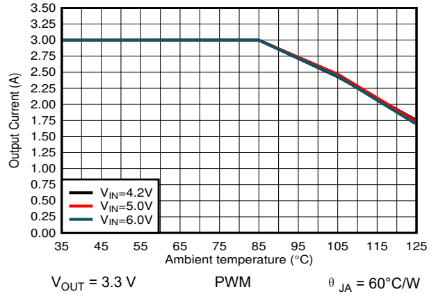
图 10-21. Output Current Versus Ambient Temperature
