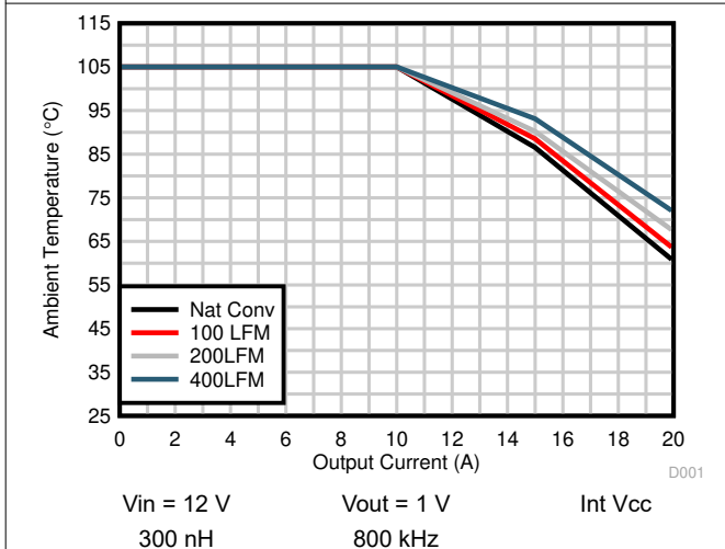
图 6-5. Safe Operating Area, V OUT = 1.0 V
