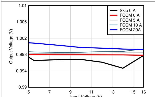
图 8-12. Output Voltage vs Input Voltage VCC = 3.3-V External Bias
