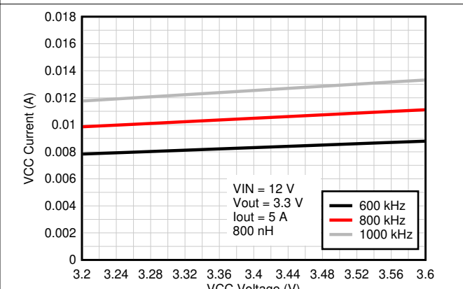
图 8-13. ICC Current vs External VCC Voltage
