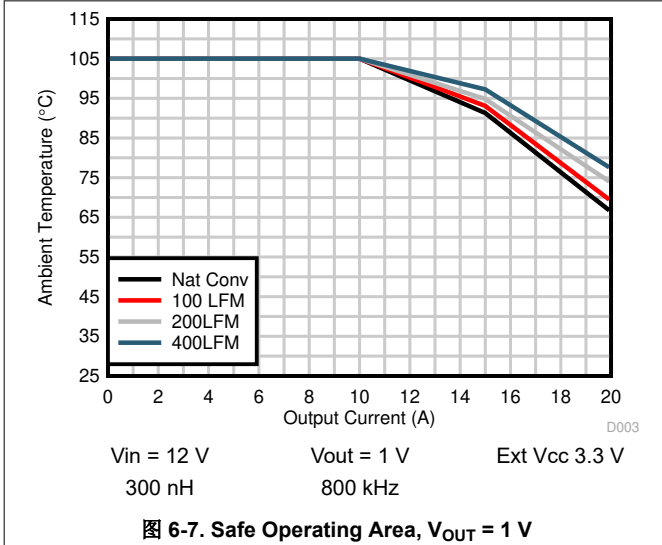
图 6-7. Safe Operating Area, V_{OUT} = 1\text{ V}
