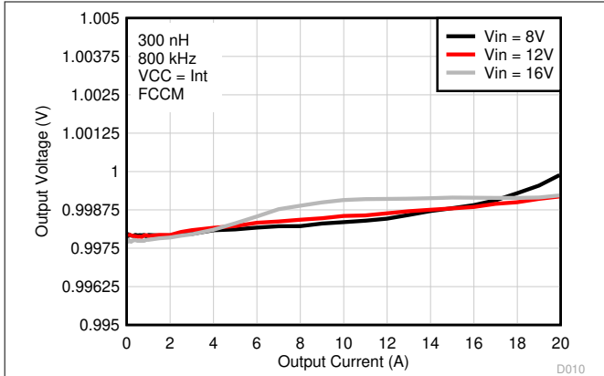
图 8-8. Output Voltage vs Output Current
