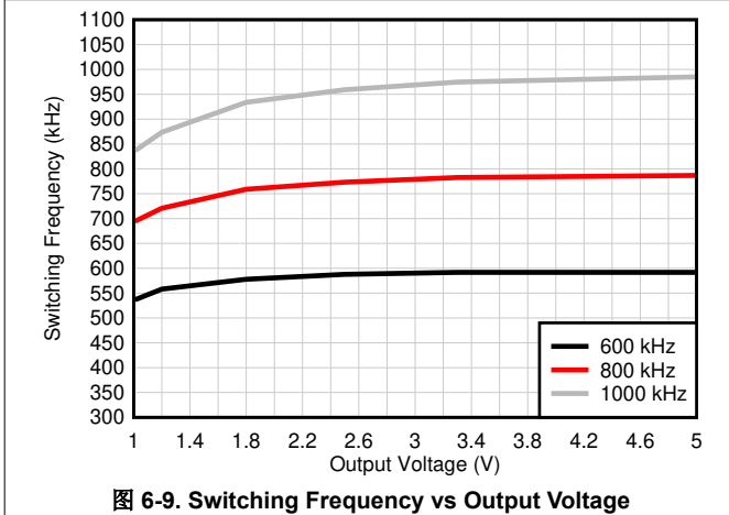
图 6-9. Switching Frequency vs Output Voltage
