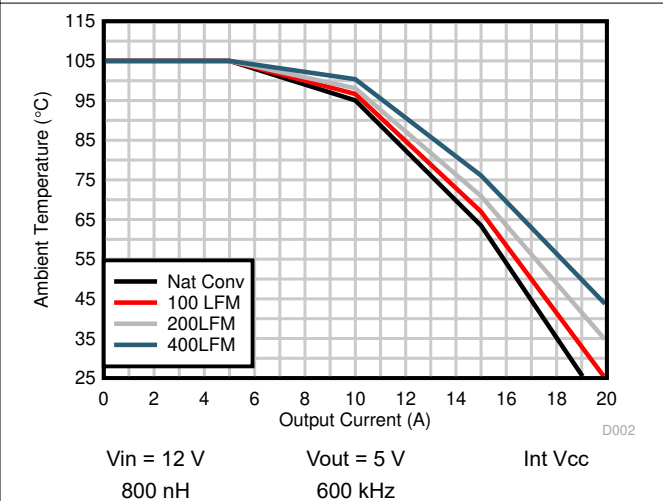
图 6-6. Safe Operating Area, V OUT = 5 V
