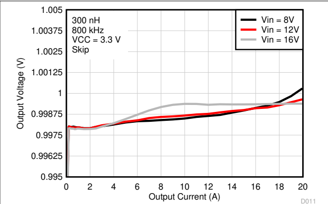
图 8-9. Output Voltage vs Output Current, VCC = 3.3-V External Bias
