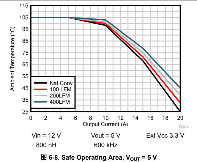
图 6-8. Safe Operating Area, V_{OUT} = 5\text{ V}
