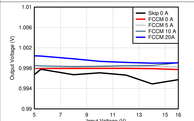
图 8-11. Output Voltage vs Input Voltage VCC = Int
