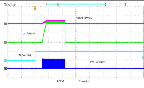
图 8-29. Enabled into Overcurrent
