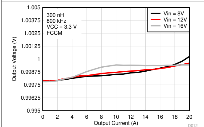
图 8-10. Output Voltage vs Output Current, VCC = 3.3-V External Bias
