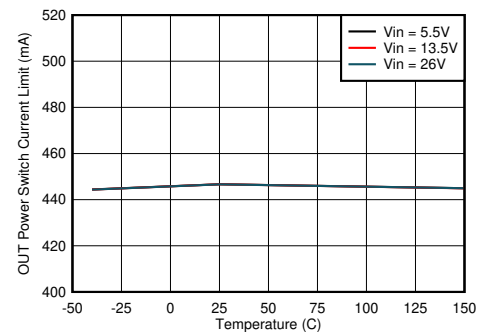
图 8-14. OUT Power Switch Current Limit vs Junction Temperature
