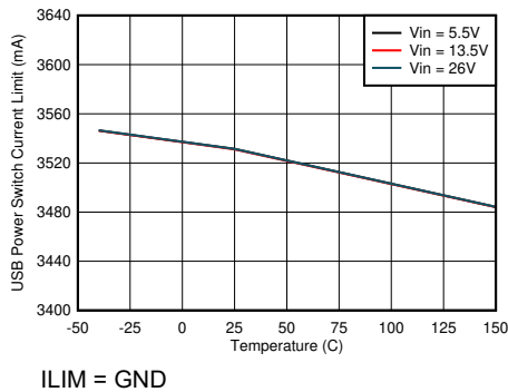
图 8-11. USB Power Switch Current Limit vs Junction Temperature
