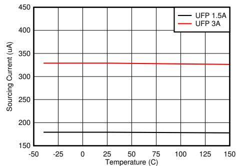
图 8-22. CC Sourcing Current vs Junction Temperature
