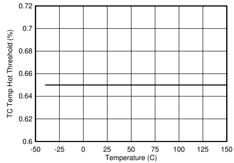
图 8-24. TS Temperature Hot Threshold vs Junction Temperature
