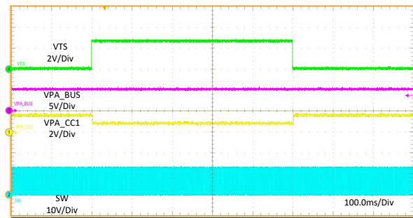
图 11-30. Thermal Sensing - NTC Temperature WARM Behavior
