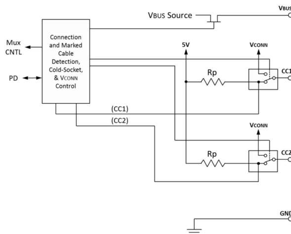
图 10-15. Source Functional Model for CC1 and CC2 (From Type-C Specification)
