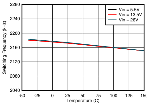
图 8-21. Switching Frequency vs Junction Temperature
