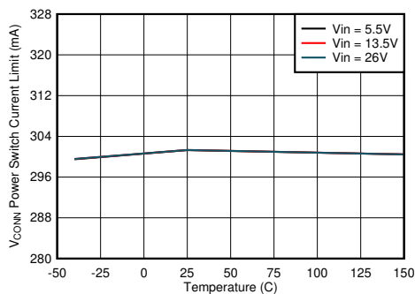
图 8-15. V_{CONN} Power Switch Current Limit vs Junction Temperature
