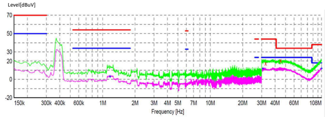
图 11-4. 400-kHz EMI Results (Without CM Filter)
