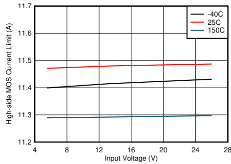
图 8-7. High-side Current Limit vs Input Voltage
