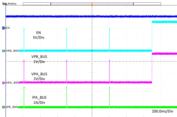
图 11-25. 1- \Omega Load Recovery
