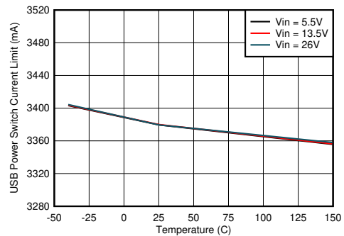
图 8-12. USB Power Switch Current Limit vs Junction Temperature
