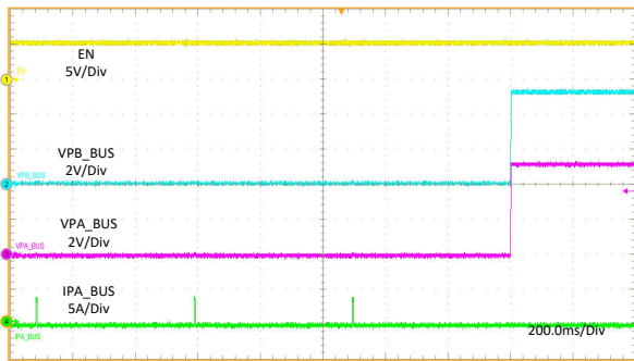
图 11-23. Short Circuit Recovery
