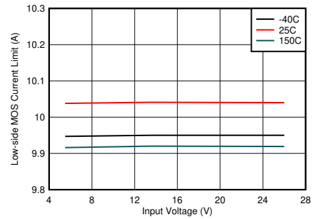
图 8-8. Low-side Current Limit vs Input Voltage
