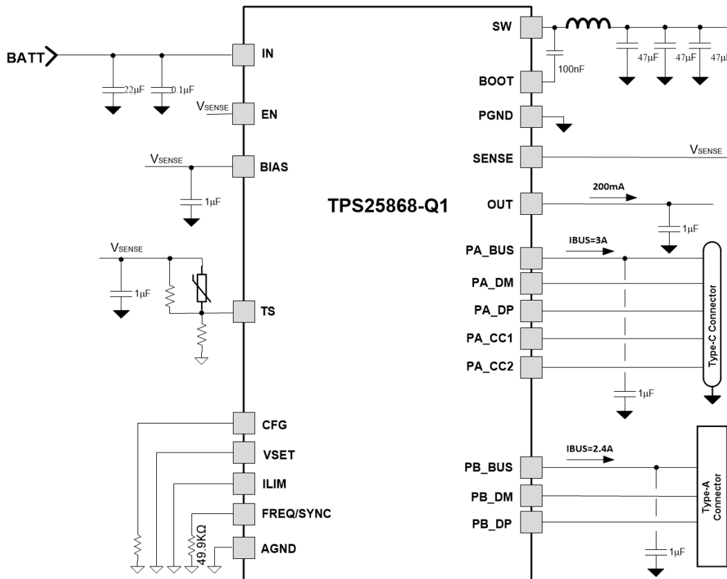
图 11-1. TPS25868-Q1 Typical Application Circuit for 400-kHz f_{sw}
