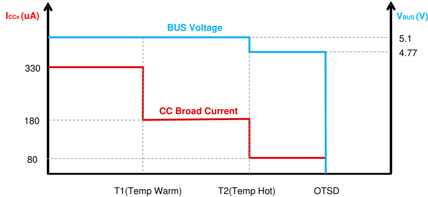
图 10-11. TPS2586x-Q1 Behavior When Trigger Temp Warm and Hot threshold
