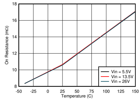
图 8-10. Low-side MOSFET on Resistance vs Junction Temperature
