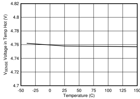
图 8-25. SENSE Voltage in Temperature Hot vs Junction Temperature
