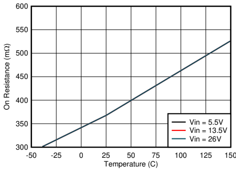
图 8-19. V CONN Power Switch On Resistance vs Junction Temperature
