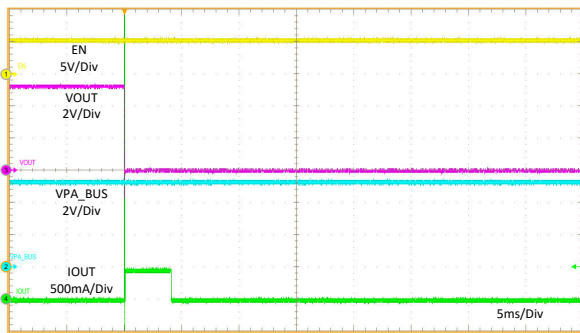
图 11-27. PA_CC2 Hot Short to GND
