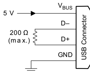
图 10-16. DCP Supporting BC1.2 and YD/T 1591-2009
