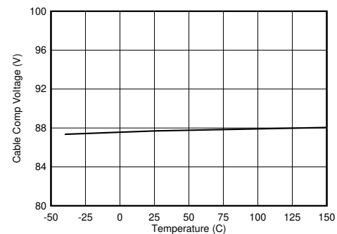
图 8-16. Cable Compensation Voltage vs Junction Temperature
