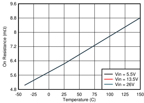
图 8-17. USB Power Switch On Resistance vs Junction Temperature
