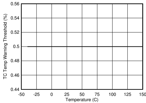
图 8-23. TS Temperature Wam Threshold vs Junction Temperature
