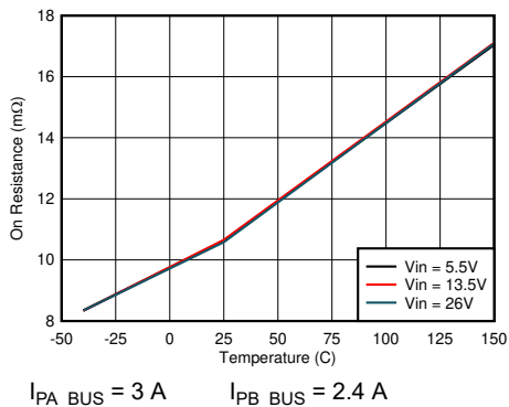
图 8-11. Low-side MOSFET on Resistance vs Junction Temperature
