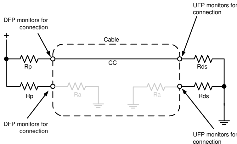
图 10-20. DFP-UFP Connection
