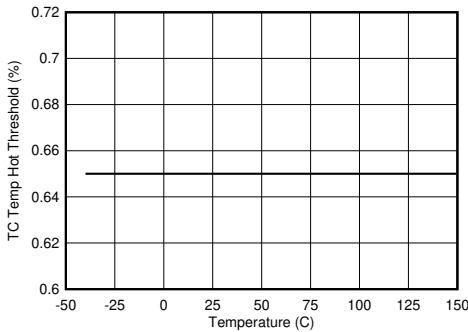
图 8-25. TS Temperature Hot Threshold vs Junction Temperature
