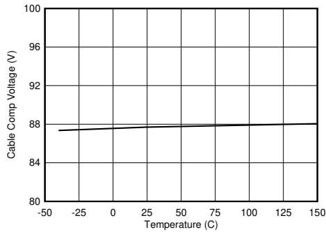
图 8-17. Cable Compensation Voltage vs Junction Temperature
