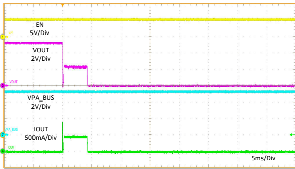
图 11-29. OUT Short to 5.1-Ω Load
