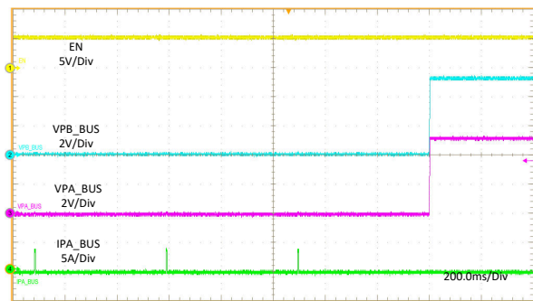
图 11-24. Short Circuit Recovery
