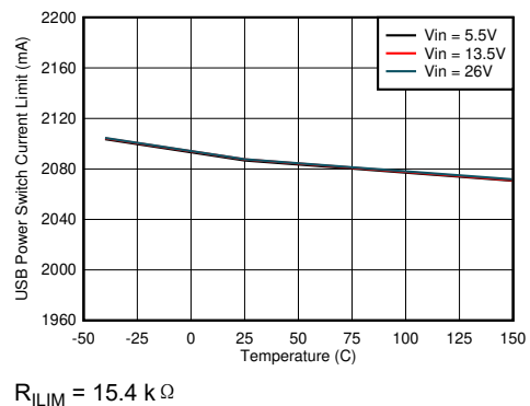
图 8-14. USB Power Switch Current Limit vs Junction Temperature
