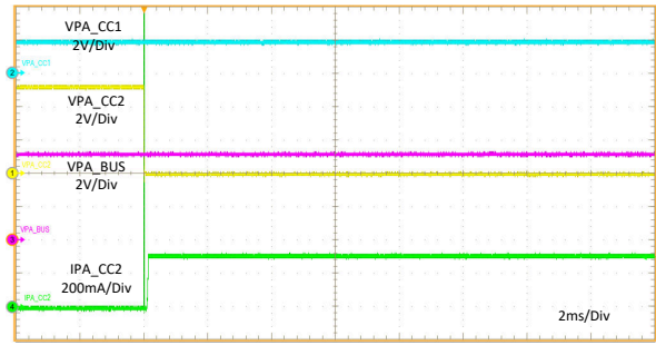
图 11-28. PA_CC2 Hot Short to GND
