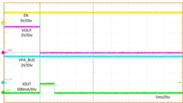
图 11-28. PA_CC2 Hot Short to GND
