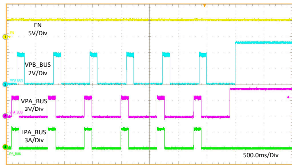
图 11-26. 1- \Omega Load Recovery
