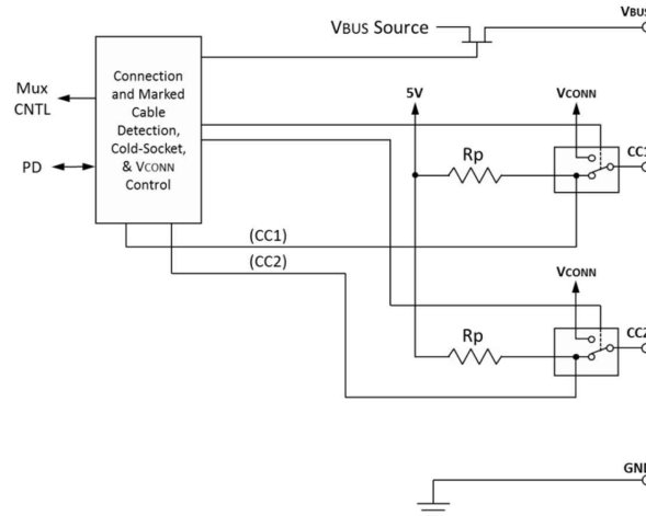
图 10-21. Source Functional Model for CC1 and CC2 (From Type-C Specification)
