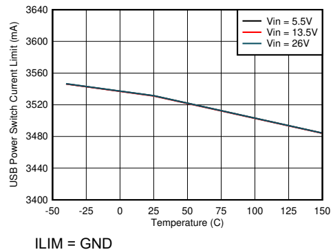
图 8-12. USB Power Switch Current Limit vs Junction Temperature
