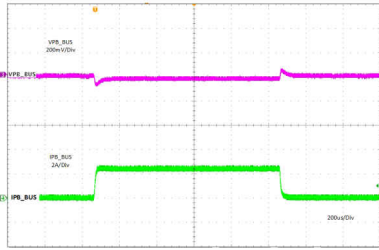
图 11-9. Load Transient Without Cable Compensation
