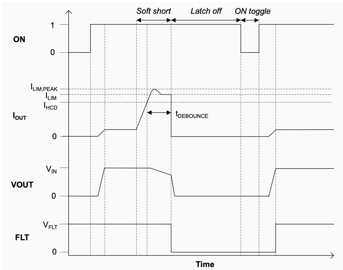
图 9-3. Output Current Limit Behavior
