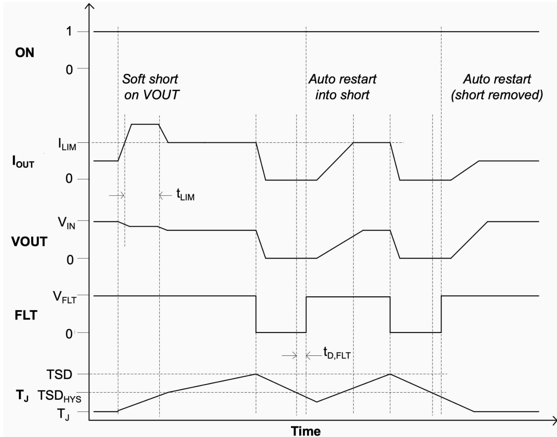
图 9-1. Output Current Limit for Short-Circuit Protection ( t_{LIM} )
