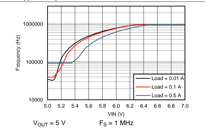
Figure 20. Switching Frequency vs V_{IN} in Dropout Operation
