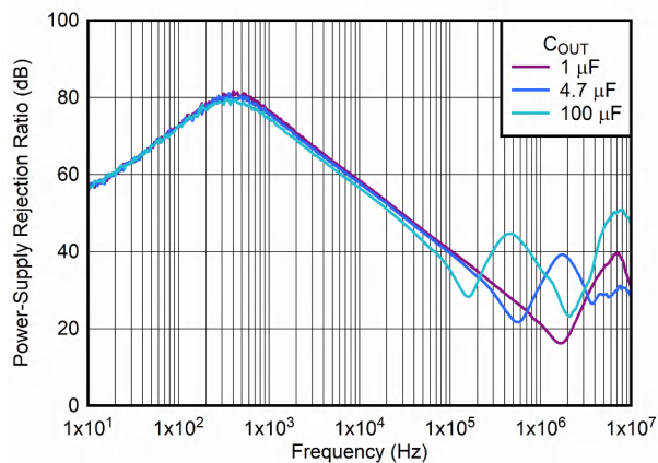
图 6-23. V_{IN} PSRR vs Frequency and C_{OUT}
