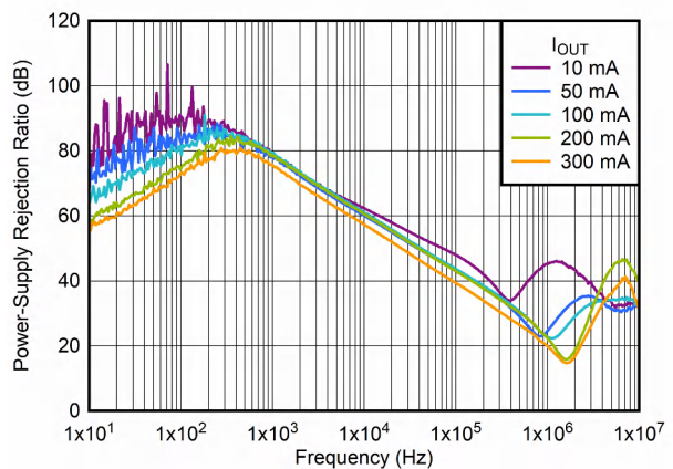
图 6-24. V_{IN} PSRR vs Frequency and I_{OUT}
