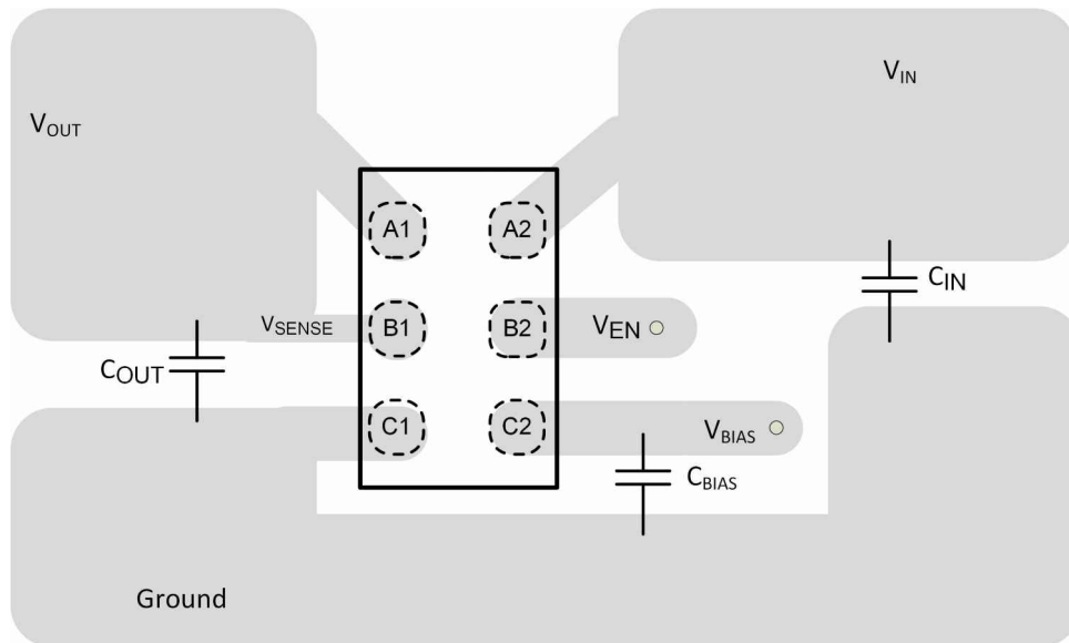
图 10-1. Recommended Layout
