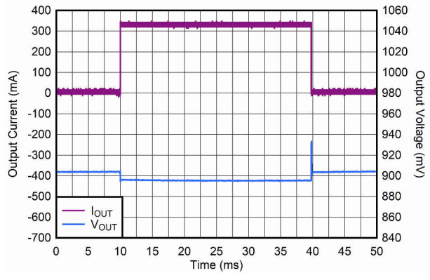
图 6-20. Load Transient From 100 \mu\text{A} to 320 mA
