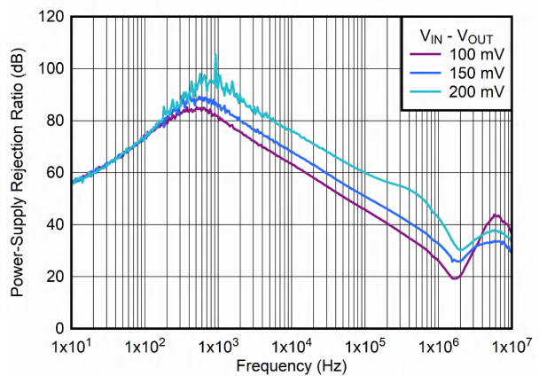
图 6-22. V_{IN} PSRR vs Frequency and V_{IN} - V_{OUT}
