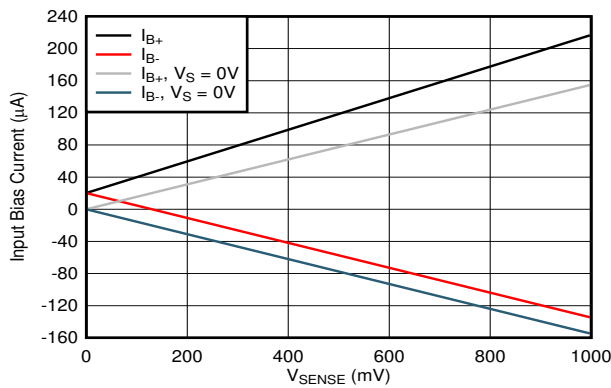
图 6-15. Input Bias Current vs V_{\text{SENSE}} , A1 Devices
