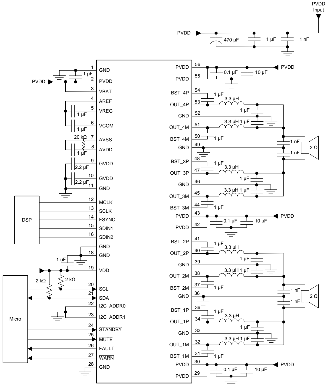
图 82. TAS6424M-Q1 Typical 2-Channel PBTL Application Schematic
