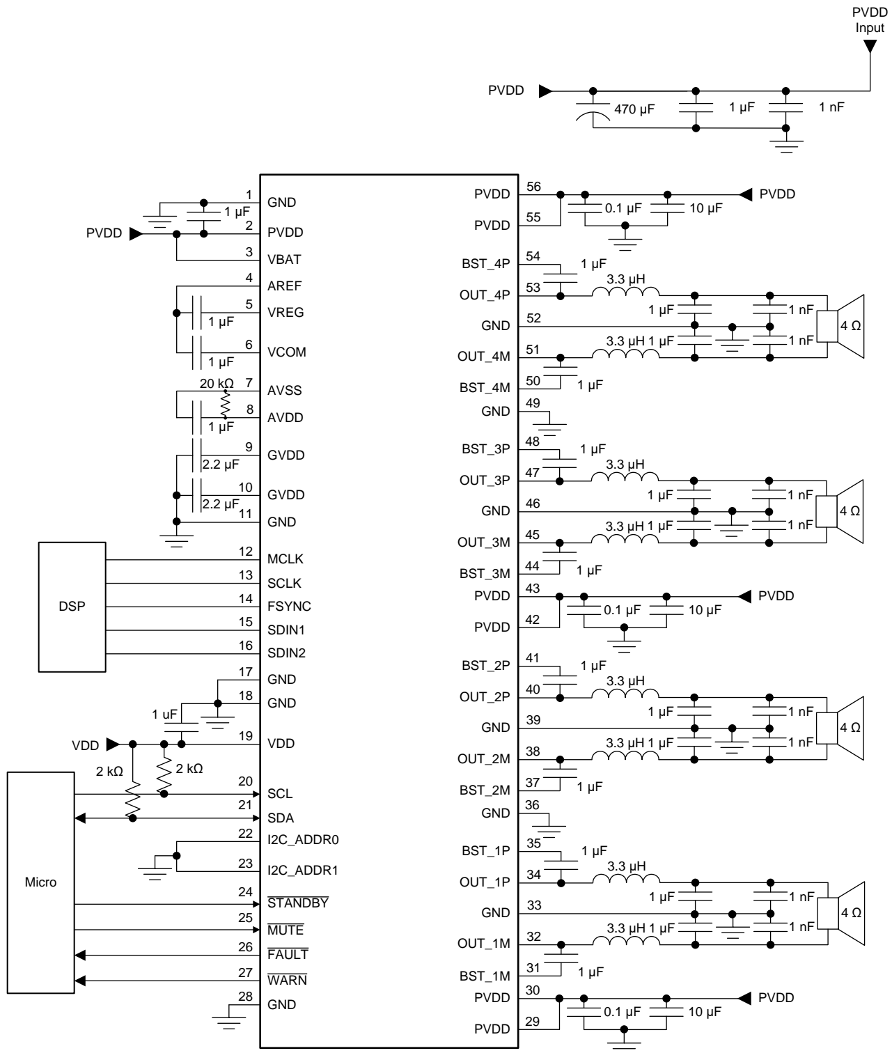
图 79. TAS6424M-Q1 Typical 4-Channel BTL Application Schematic
