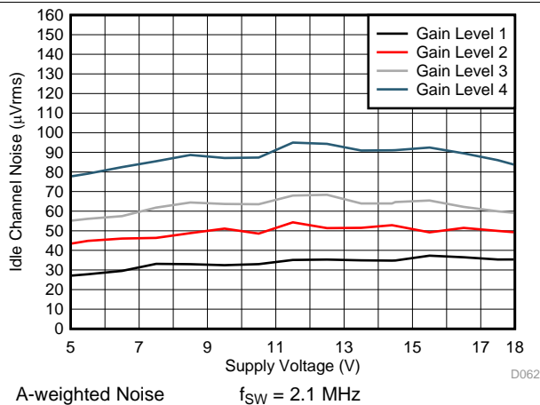
图 11. Noise vs Supply voltage
