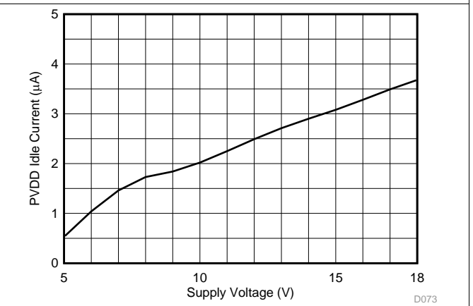
图 16. PVDD Idle Current vs Voltage
