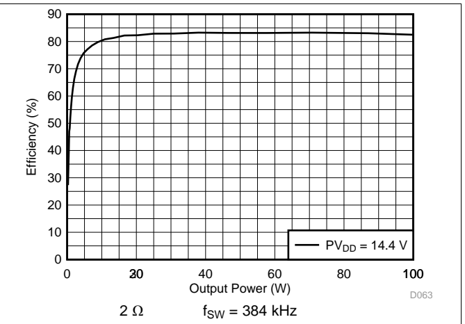
图 14. PVDD Power Efficiency vs Total Output Power
