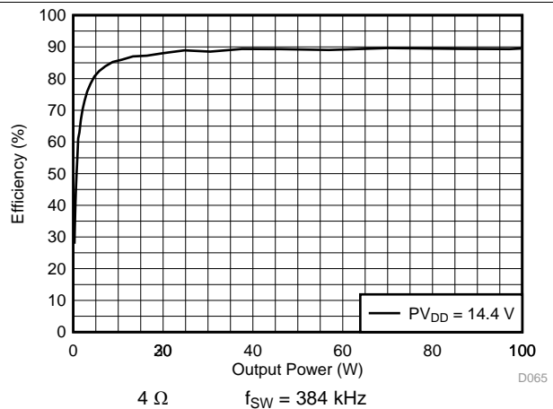
图 12. PVDD Power Efficiency vs Total Output Power
