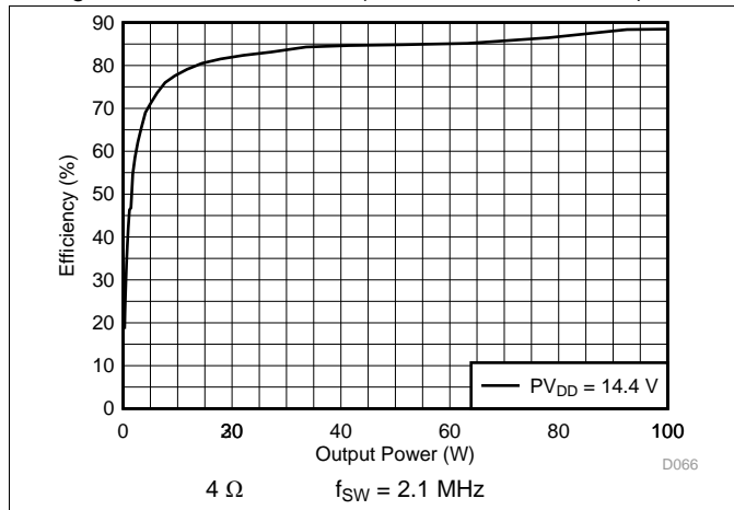
图 13. PVDD Power Efficiency vs Total Output Power
