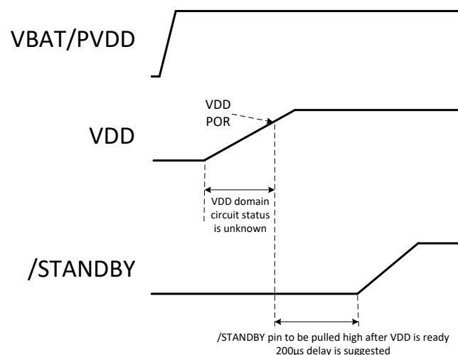
图 40. Power-Up Sequence Option 2
