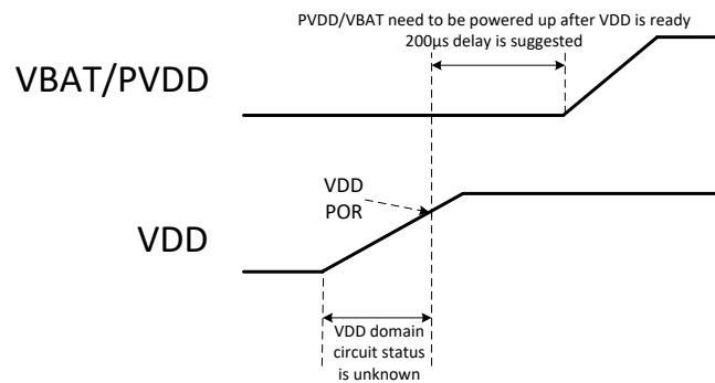
图 39. Power-Up Sequence Option 1
