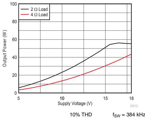
图 9. Output Power vs Supply Voltage
