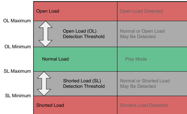
图 36. DC Load Diagnostic Reporting Thresholds
