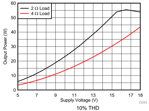
图 10. Output Power vs Supply Voltage
