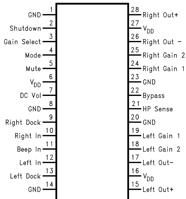
Figure 2. HTSSOP Package (Top View) See Package Number PWP0028A for HTSSOP
