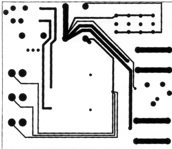
Figure 51. Bottom Layer TSSOP
