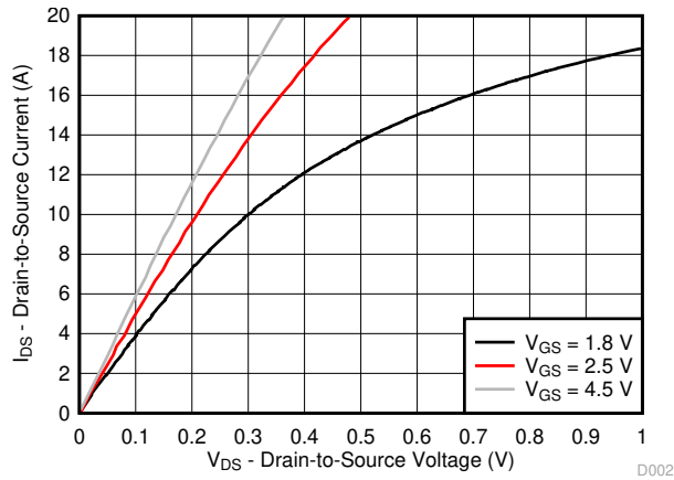
图 5-1. Saturation Characteristics
