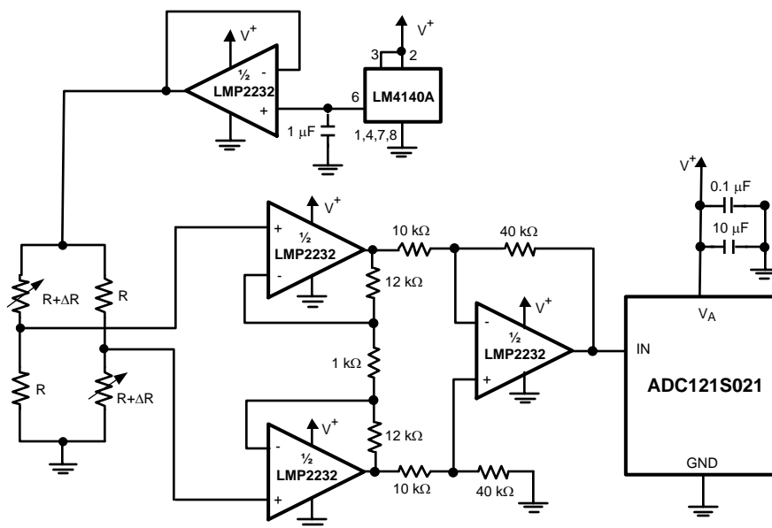
Figure 51. Strain Gage Bridge Amplifier
