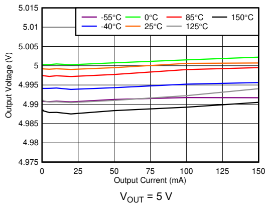
V_{OUT} = 5\ \text{V} 图 6-5. Load Regulation vs I_{OUT}
