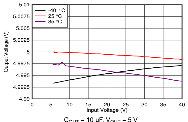
C_{OUT} = 10\ \mu\text{F} , V_{OUT} = 5\ \text{V} 图 6-6. Line Regulation at 50 mA
