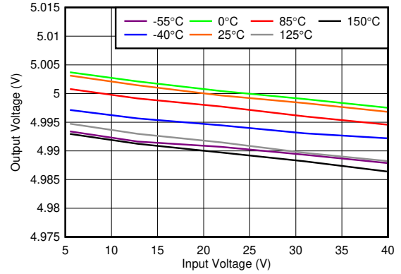
V_{OUT} = 5\ \text{V} , I_{OUT} = 150\ \text{mA} 图 6-2. Line Regulation vs V_{IN}
