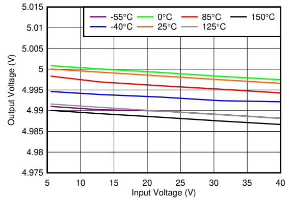
V_{OUT} = 5\ \text{V} , I_{OUT} = 1\ \text{mA} 图 6-4. Line Regulation vs V_{IN}
