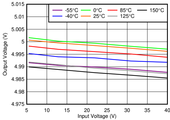
V_{OUT} = 5\ \text{V} , I_{OUT} = 5\ \text{mA} 图 6-3. Line Regulation vs V_{IN}
