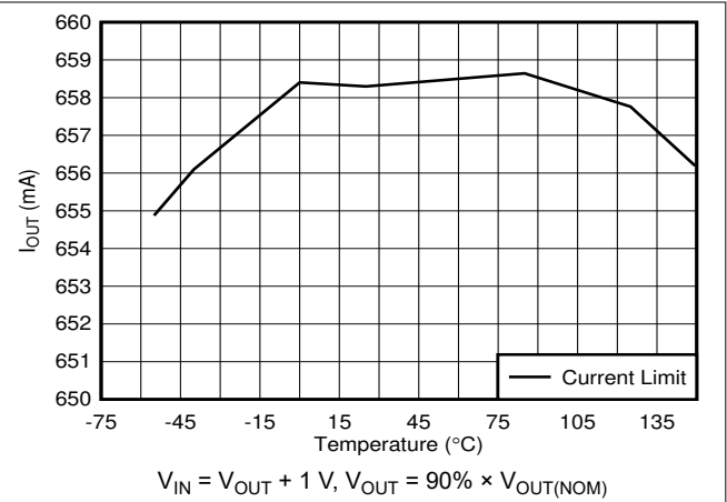
图 6-26. Output Current Limit vs Temperature
