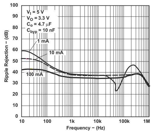
图 6-22. Ripple Rejection vs Frequency for Legacy Chip
