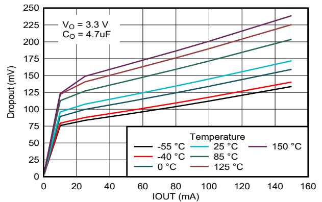
图 6-4. Dropout Voltage vs Temperature for Legacy Chip
