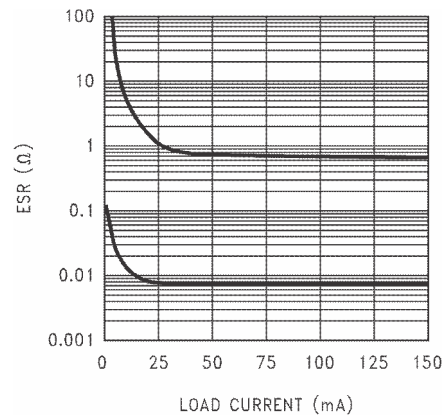
图 6-36. 2.2-µF Stable ESR Range for Output Voltage \leq 2.3\text{ V} for Legacy Chip
