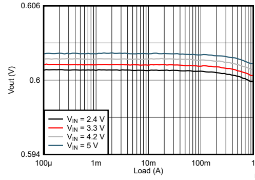
图 9-42. Load Regulation
