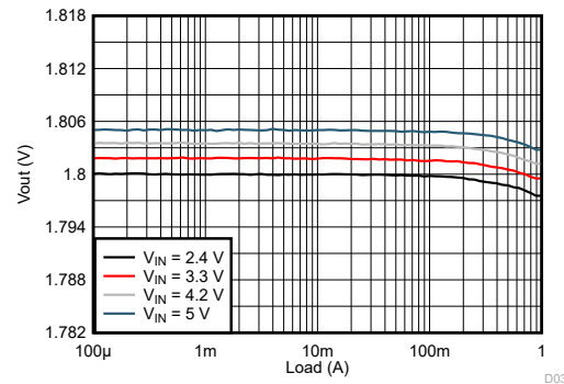
图 9-42. Load Regulation
