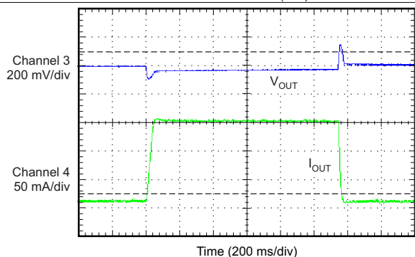
V_{IN} = 5\text{ V} , V_{OUT} = 1.8\text{ V} , C_{IN} = C_{OUT} = 0\text{ }\mu\text{F}
