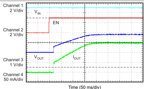
V_{IN} = 3\text{ V} , I_{OUT} = 150\text{ mA} , V_{OUT} = 1.8\text{ V} , C_{IN} = C_{OUT} = 0\text{ }\mu\text{F}
