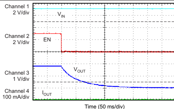
V_{IN} = 3\text{ V} , I_{OUT} = 0\text{ mA} , V_{OUT} = 1.8\text{ V} , C_{IN} = C_{OUT} = 1\text{ }\mu\text{F}
