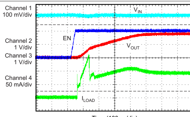
V_{IN} = 2.3\text{ V} , I_{OUT} = 90\text{ mA} , C_{OUT} = 10\text{ }\mu\text{F} , V_{OUT} = 1.8\text{ V} , C_{IN} = 1\text{ }\mu\text{F}
