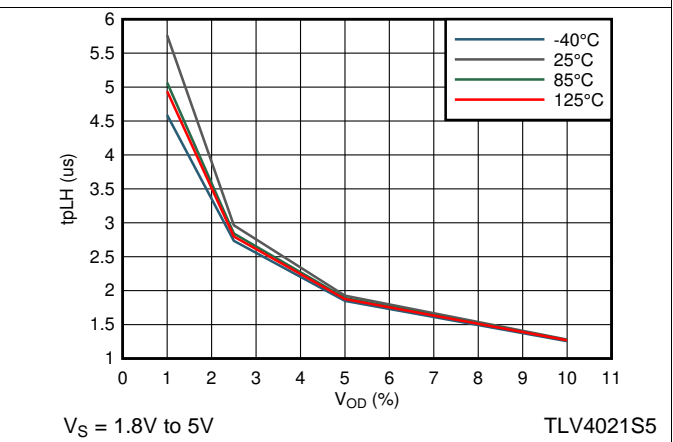
图 32. Propagation Delay Low-High vs Input Overdrive
