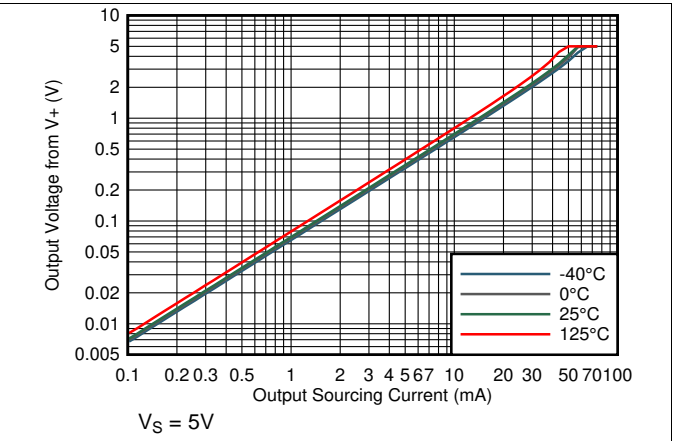
图 28. Output Voltage vs Output Sourcing Current
