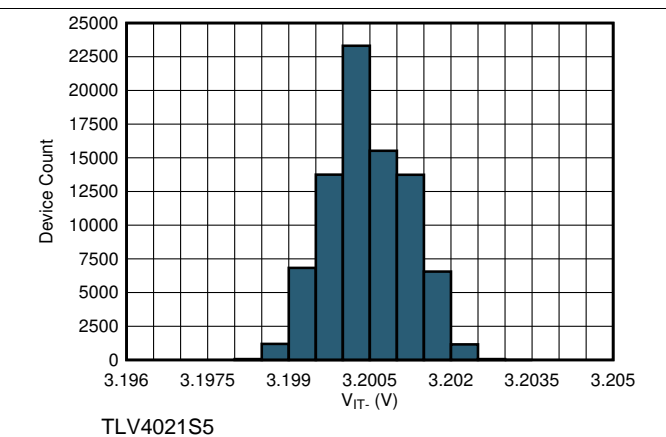
图 18. Negative Threshold Histogram
