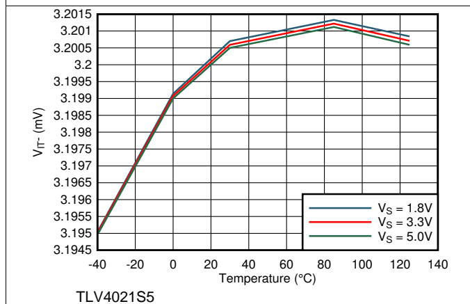
图 17. Negative Threshold vs Temperature
