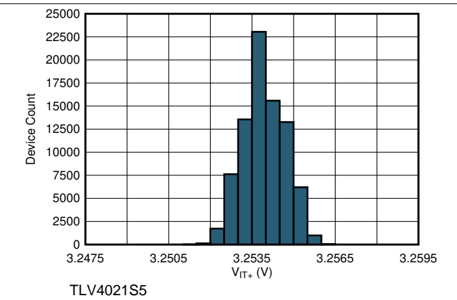
图 16. Positive Threshold Histogram
