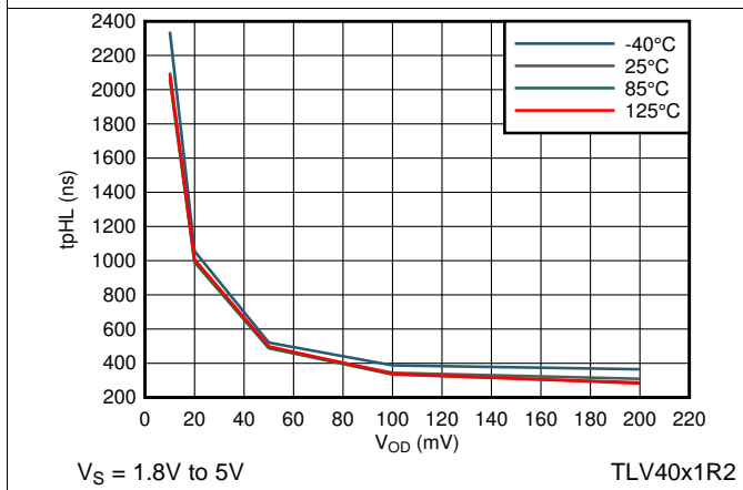
图 31. Propagation Delay High-Low vs Input Overdrive
