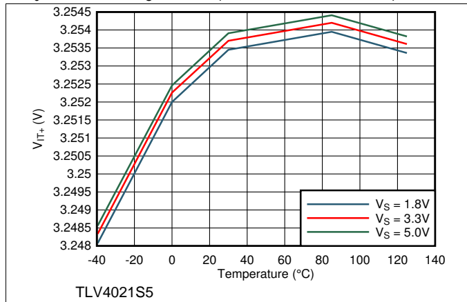
图 15. Positive Threshold vs Temperature
