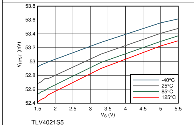
图 19. Hysteresis vs Supply Voltage
