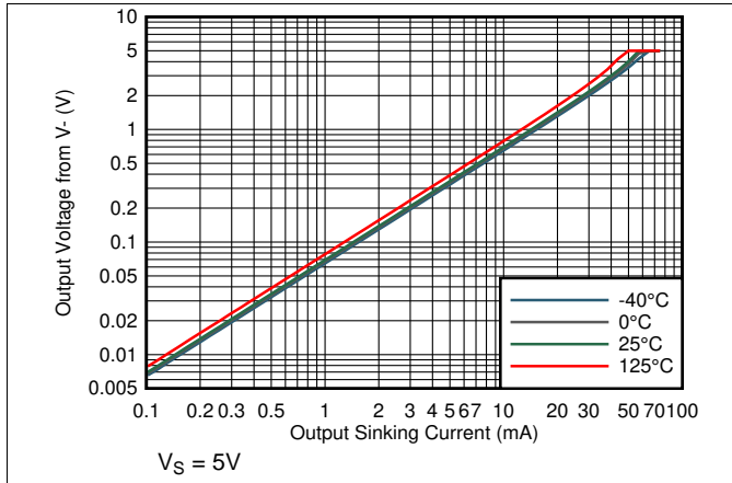
图 27. Output Voltage vs Output Sinking Current
