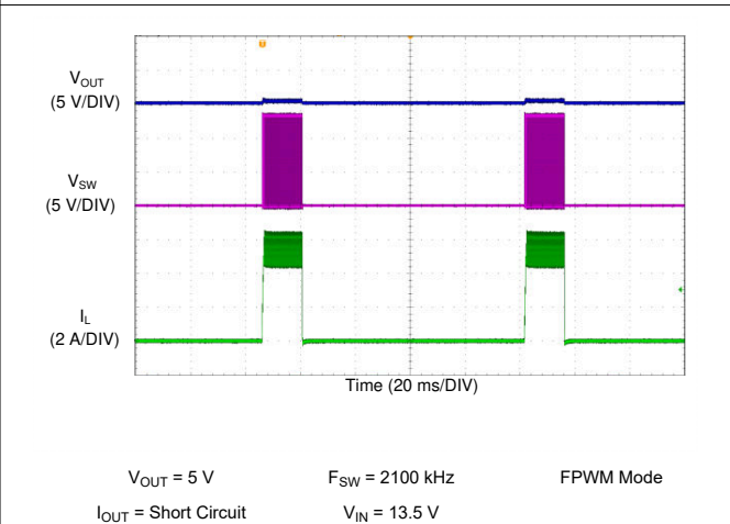
图 9-22. LM62435-Q1 Short Circuit Performance
