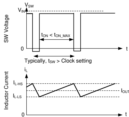
图 8-18. Current Limit Waveforms
