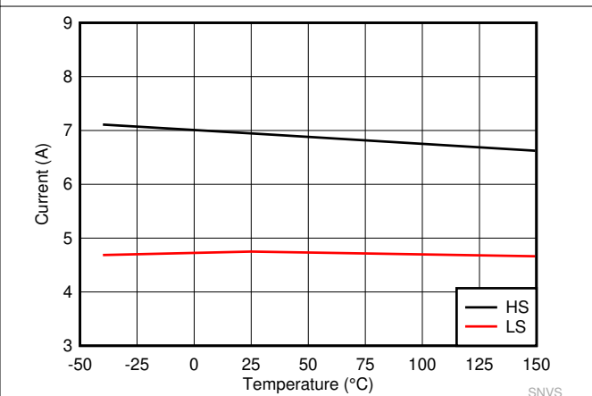
图 7-4. LM62435-Q1 High-side and Low-side Current Limits
