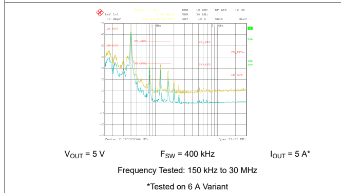
图 9-25. Conducted EMI versus CISPR25 Limits (Yellow: Peak Signal, Blue: Average Signal)
