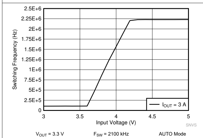
图 9-15. LM62435-Q1 Frequency Dropout Curve
