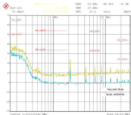
传导 EMI：V OUT =5V，f SW =2100kHz
