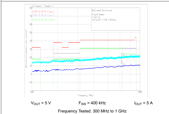
图 9-31. Radiated EMI Log Horizontal versus CISPR25 Limits
