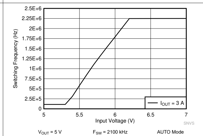
图 9-16. LM62435-Q1 Frequency Dropout Curve
