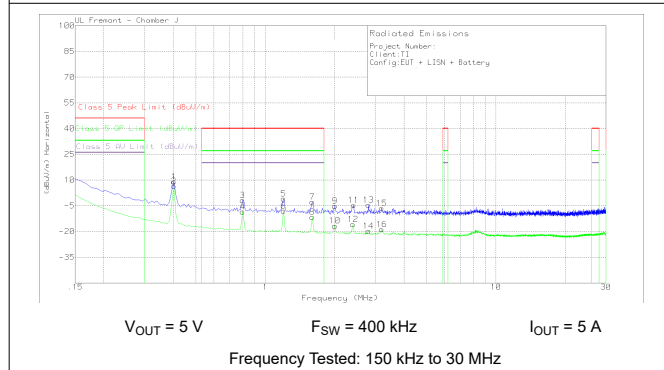
图 9-27. Radiated EMI Rod versus CISPR25 Limits
