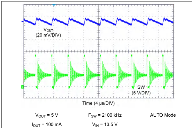
图 9-17. LM62435-Q1 Switching Waveform and V_{OUT} Ripple
