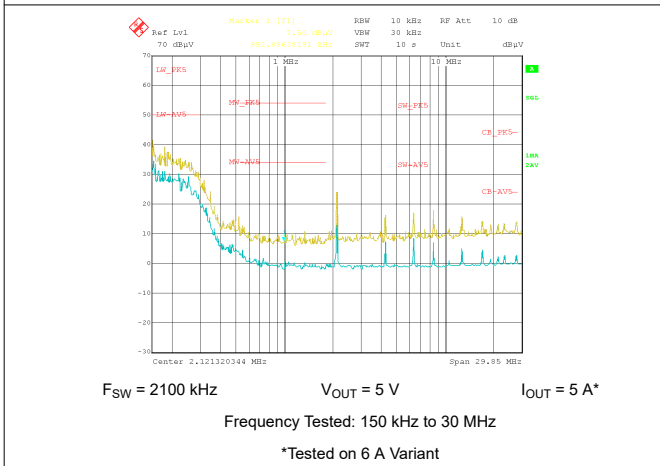
图 9-33. Conducted EMI versus CISPR25 Limits (Yellow: Peak Signal, Blue: Average Signal)
