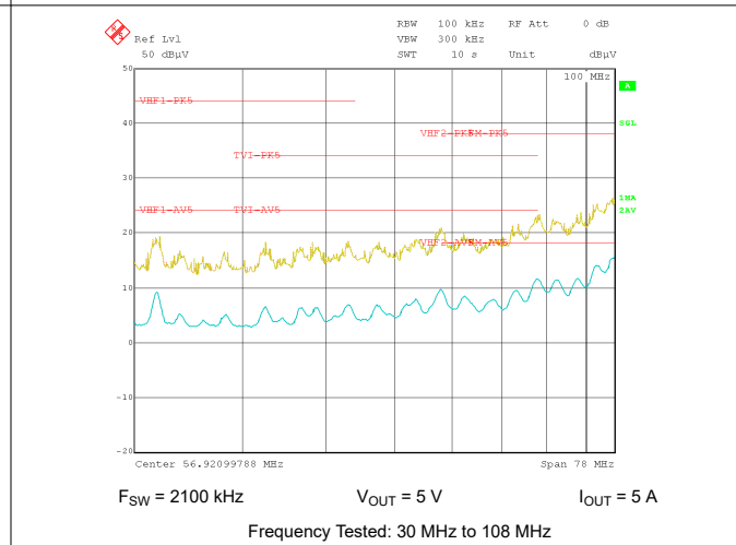
图 9-34. Conducted EMI versus CISPR25 Limits (Yellow: Peak Signal, Blue: Average Signal)
