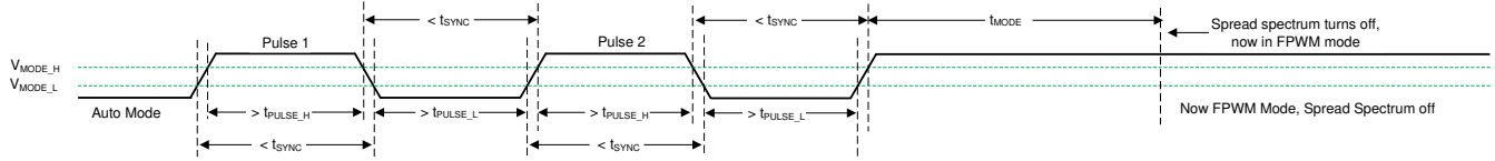
图 8-9. Spread Spectrum Disabled in Transition from Auto Mode to FPWM Mode
