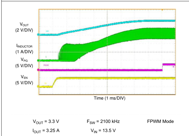
图 9-19. LM62435-Q1 Start-up with 3.25 A
