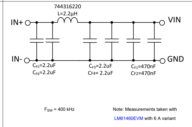
图 9-32. Recommended Input EMI Filter
