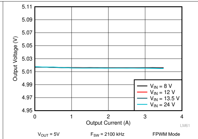
图 9-12. LM62435-Q1 Load and Line Regulation
