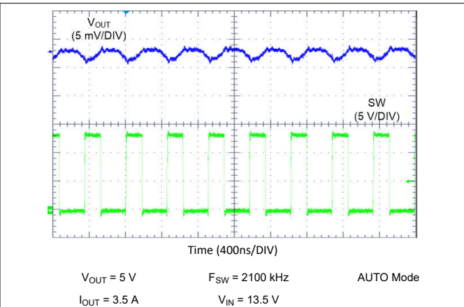
图 9-18. LM62435-Q1 Switching Waveform and V_{OUT} Ripple
