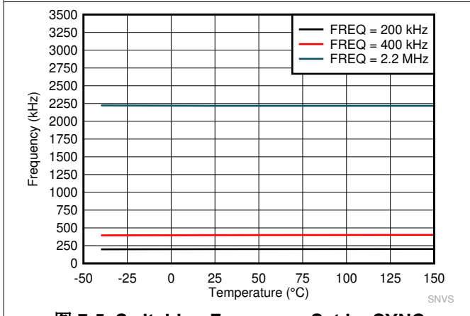
图 7-5. Switching Frequency Set by SYNC
