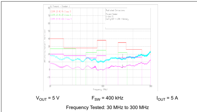
图 9-29. Radiated EMI Bicon Horizontal versus CISPR25 Limits
