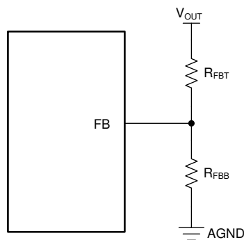
图 8-17. Setting Output Voltage of Adjustable Versions
