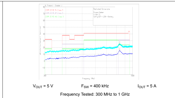
图 9-30. Radiated EMI Log Vertical versus CISPR25 Limits
