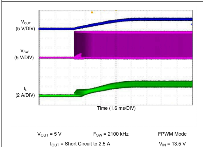
图 9-21. LM62435-Q1 Short Circuit Recovery
