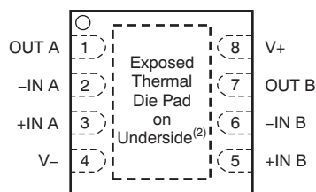
DRB Package (1) 8-Pin DFN Top View
