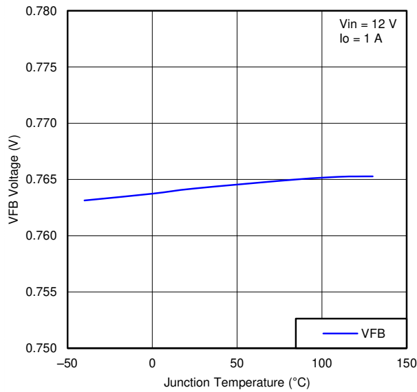
图 12-11. VFB VOLTAGE vs JUNCTION TEMPERATURE
