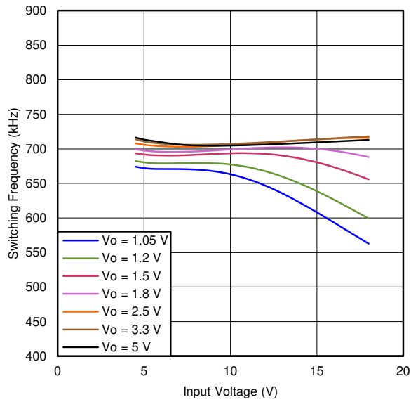
图 12-9. SWITCHING FREQUENCY vs INPUT VOLTAGE ( I_o = 1\text{ A} )
