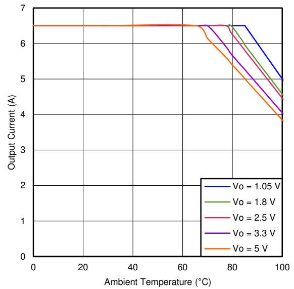
图 12-12. OUTPUT CURRENT vs AMBIENT TEMPERATURE
