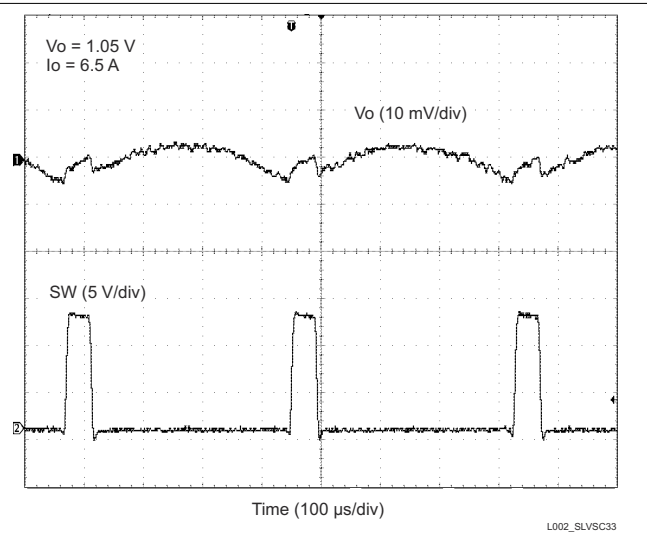
图 12-14. VOLTAGE RIPPLE AT OUTPUT ( I_O = 6.5\text{ A} )
