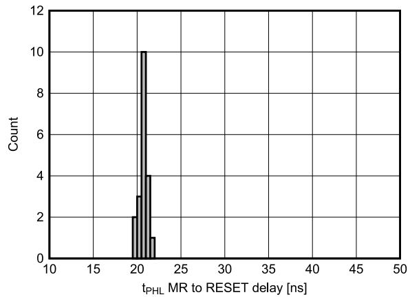
Figure 7-16. \overline{\text{MR}} to RESET ( t_{\text{PHL}} ) Delay Histogram for TPS3705-33 Devices at 25°C (Unit Count = 20)
