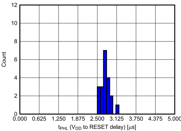
Figure 7-18. V_{\text{DD}} to RESET ( t_{\text{PHL}} ) Delay Histogram for TPS3705-33 Devices at -40°C (Unit Count = 20)
