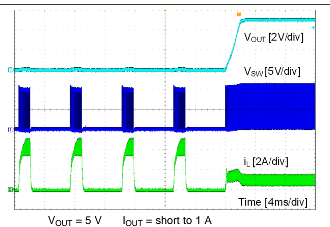
Figure 33. Short Recovery
