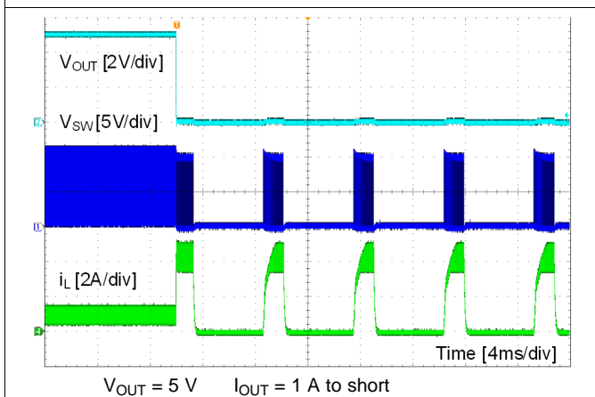
Figure 32. Short Protection
