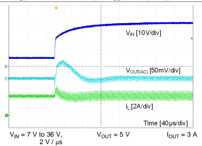
Figure 31. Line Transient
