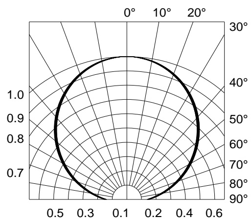
Fig.6-Radiation Diagram Ta=25°C
