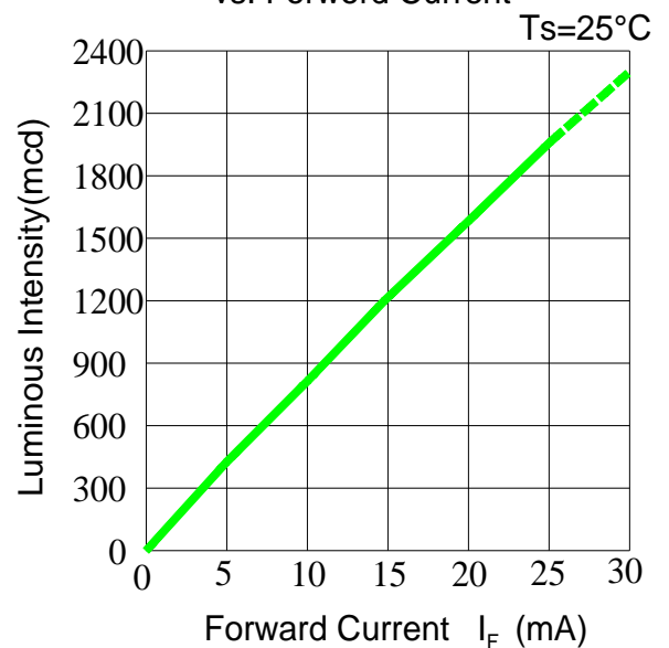
Fig.2-Luminous Intensity vs. Forward Current T s =25°C
