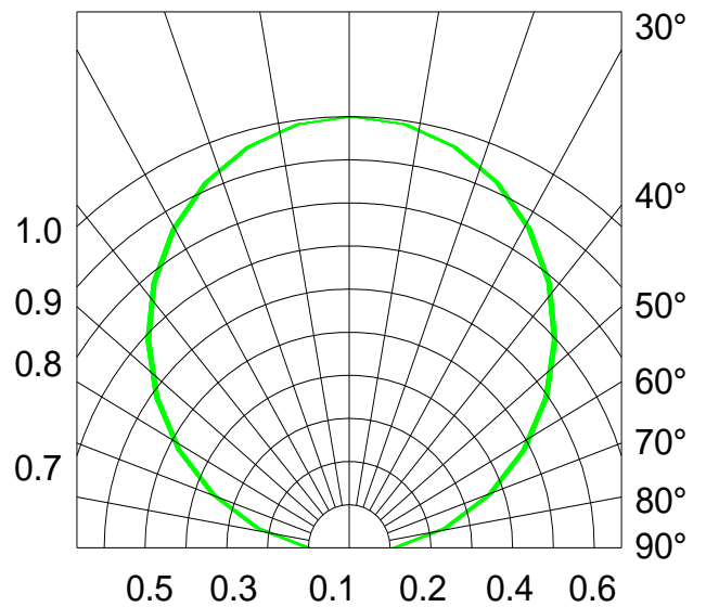
Fig.6-Radiation Diagram Ta=25°C
